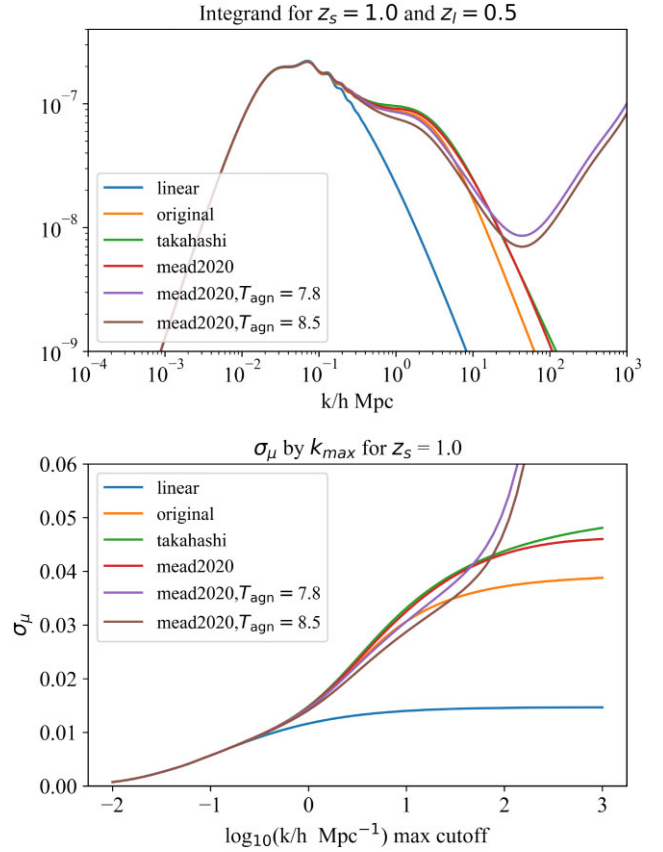
Figure 2. Upper panel. The integrand of equation (10) for a lens at z_l = 0.5 and a source at z_s = 1.0 , for a range of literature models for the matter power spectrum. The linear power spectrum is labelled as 'linear', the original halo model of Smith et al. (2003) is labelled as 'original', Takahashi et al. (2012) labelled as 'takahashi', the model of Mead et al. (2020) without baryon feedback labelled as 'mead2020', and with baryon feedback labelled according to the feedback temperature. Lower panel. \sigma_\mu as a function of the upper cut-off of the integral k_{\max} for a source at redshift z_s = 1 . It is clear that the predicted value of \sigma_\mu is sensitive to scales k/h > 1 \text{ Mpc}^{-1} . In particular, although models with baryon feedback mildly suppress the dispersion of lensing on intermediate scales, they strongly enhance it from scales k/h > 10^2 \text{ Mpc}^{-1} due to the presence of compact objects. We emphasize that this graph is for illustration only, and the non-linear models and cut-off k_{\max} do not have any role in our analysis.
