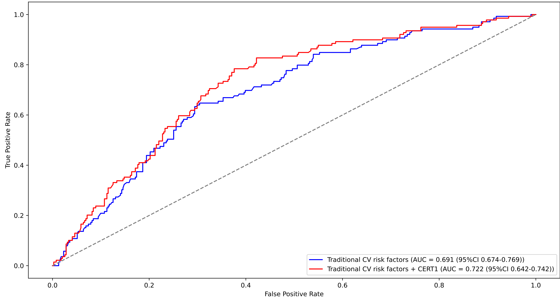
ROC curves (p-value by DeLong test = 0.0275)
