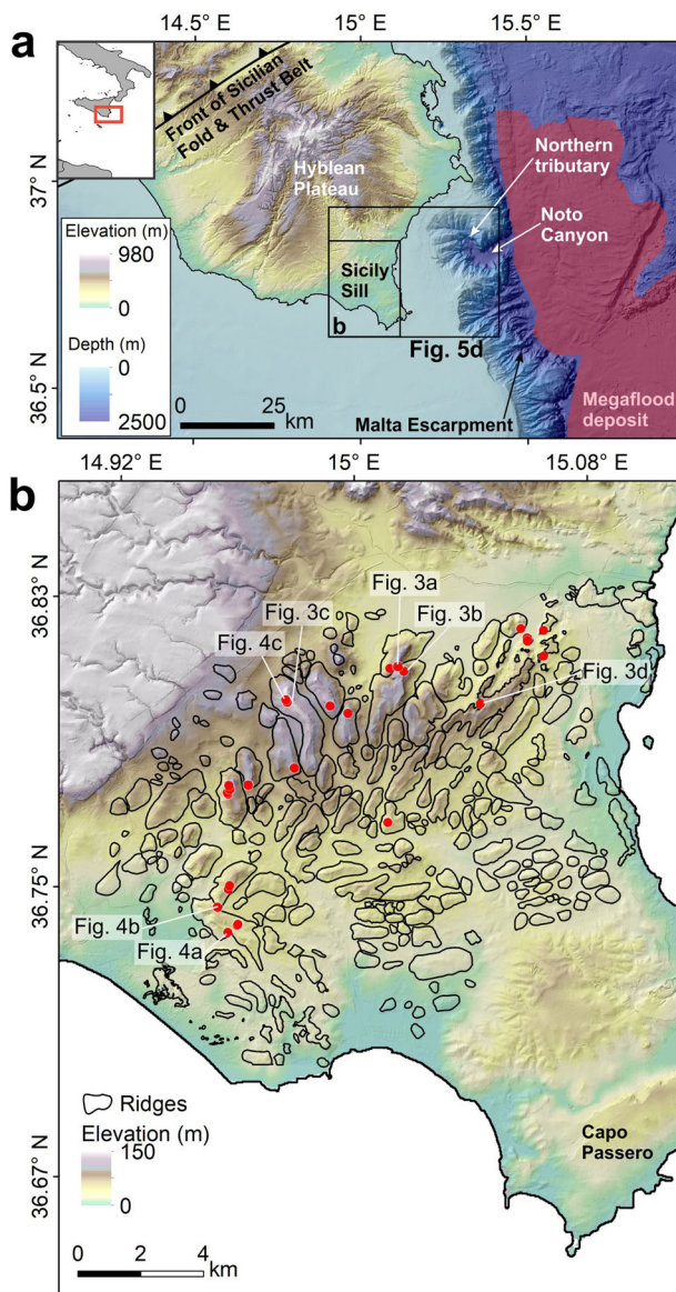
Fig. 1 | Location map. a Location map and digital elevation model of SE Sicily and adjacent seafloor (sources: SITR, EMODnet). The front of the Sicilian Fold and Thrust Belt, the Malta Escarpment, Noto Canyon, and the inferred buried megaflood deposit are labelled. b Digital elevation model of the Sicily Sill with outlines of the bases of the ridges. Sampled sites are denoted by red dots.
