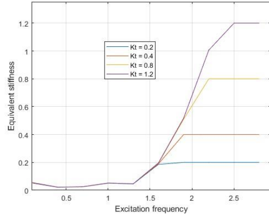
Figure 14. Variations in equivalent stiffness across different contact stiffness at A = 0.4 \text{ N}
