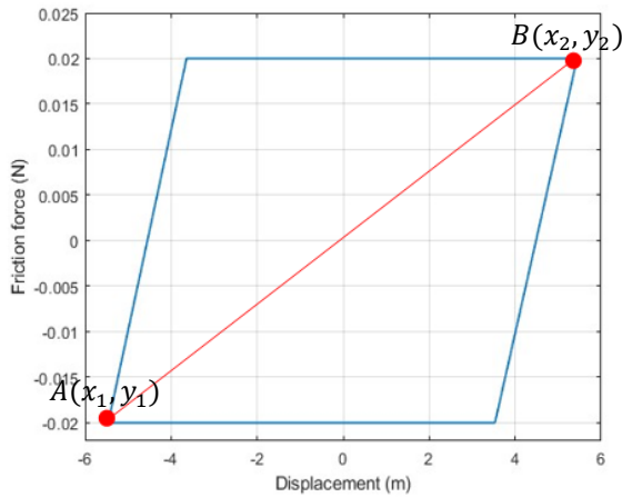
Figure 11. Hysteresis loop
