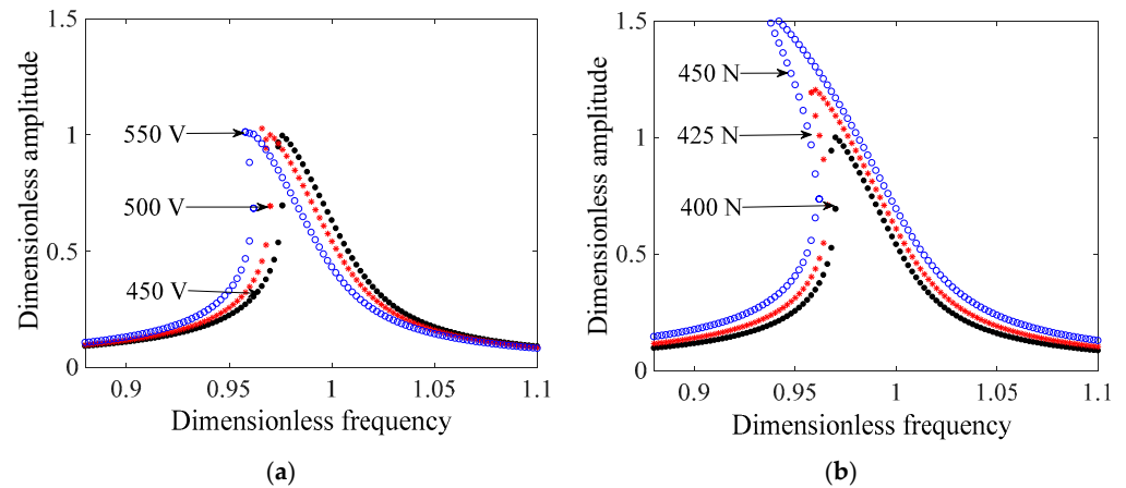
Figure 11. Frequency response characteristics of systems. (a) Frequency response characteristics under different voltage; (b) Frequency response characteristics under different preloads.
