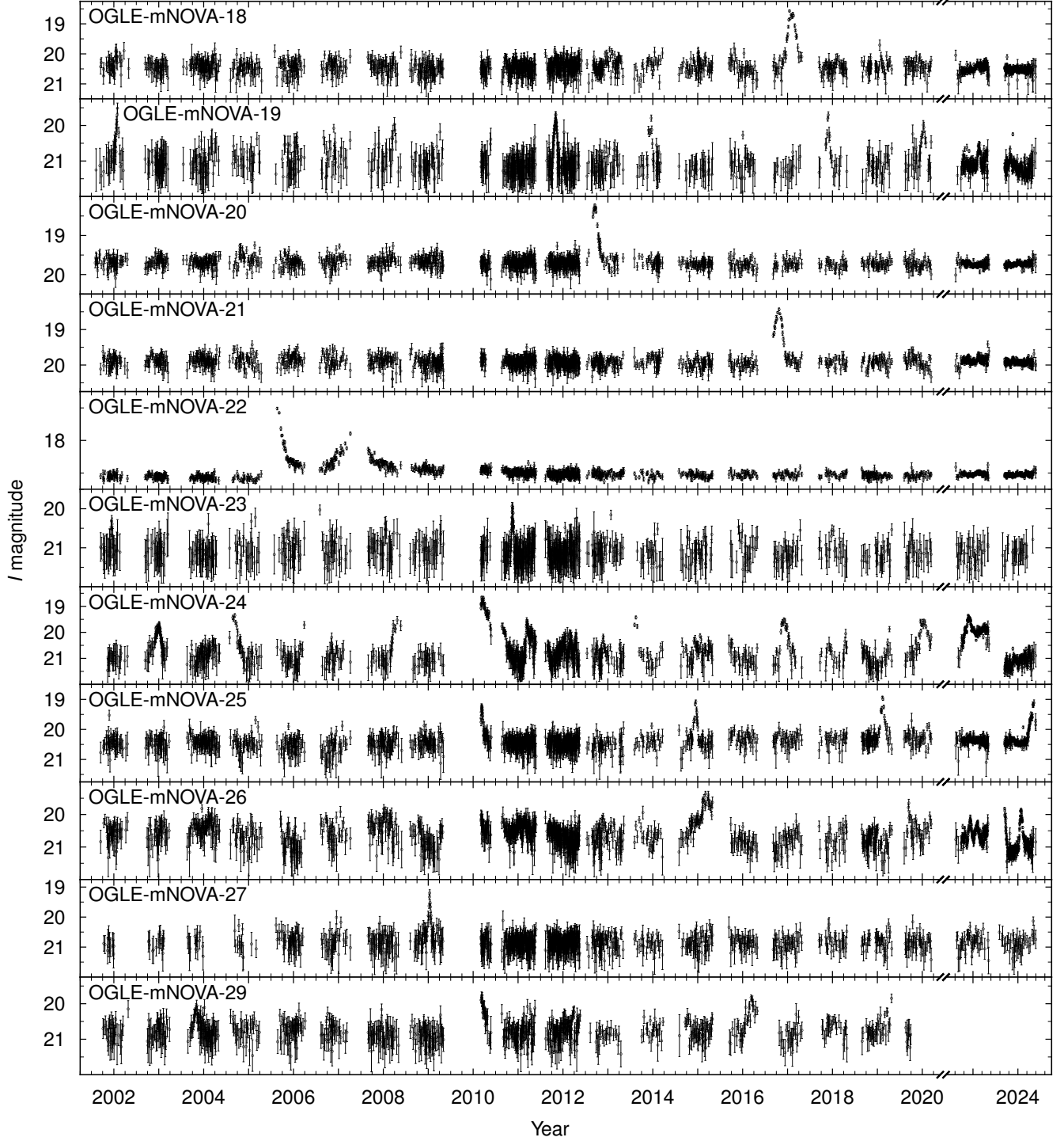
Figure A2. Example light curves of millinovae (continuation).
