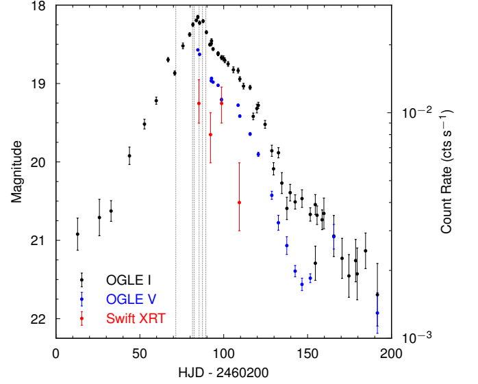
Figure 2. Photometric and X-ray observations of the 2023/2024 outburst of OGLE-mNOVA-11. Dotted lines mark times of SALT spectroscopic observations.
