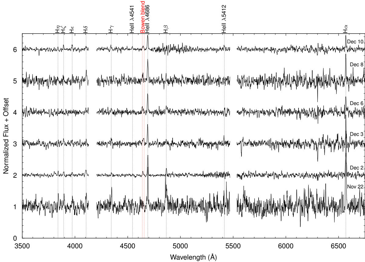
Figure 3. SALT spectroscopic observations of the 2023/2024 outburst of OGLE-mNOVA-11 reveal narrow emission lines, including He II (4686 Å) and Bowen blend.
