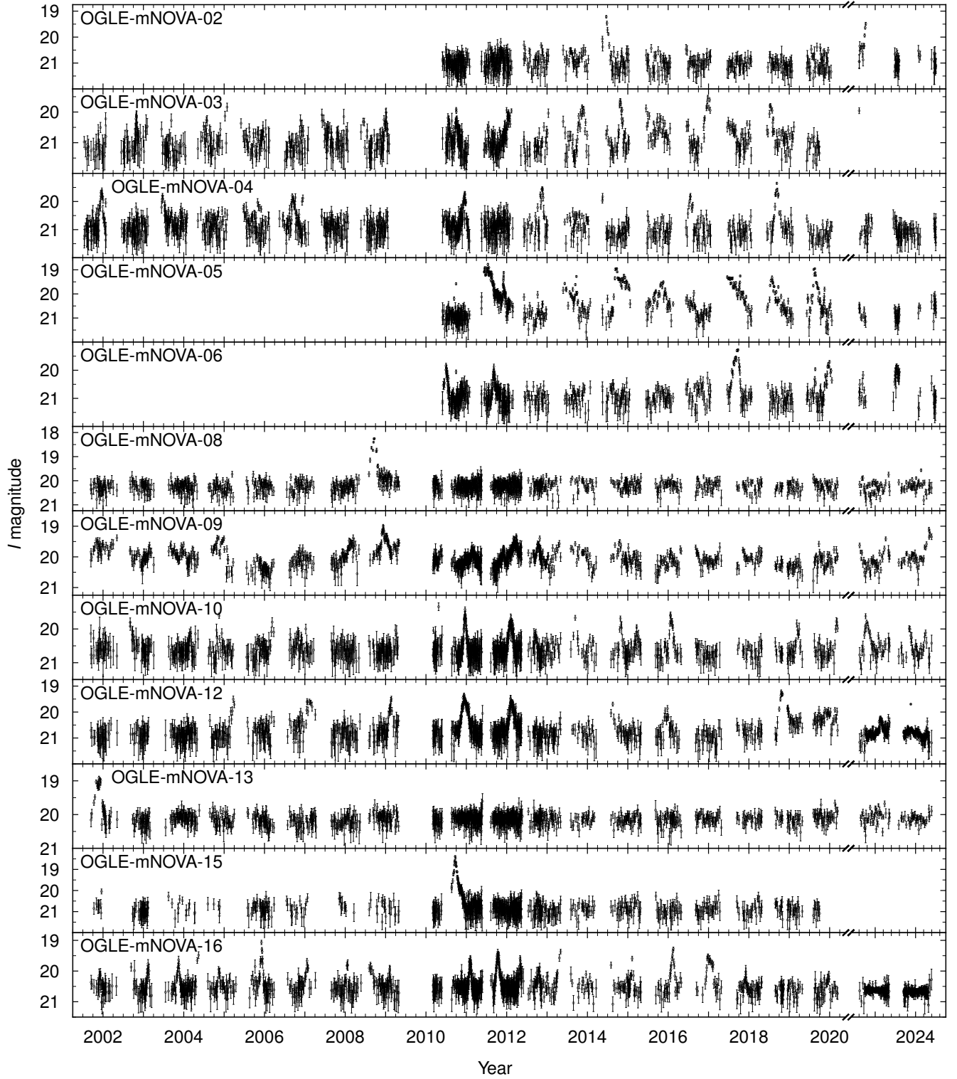
Figure A1. Example light curves of millinovae (continuation).
