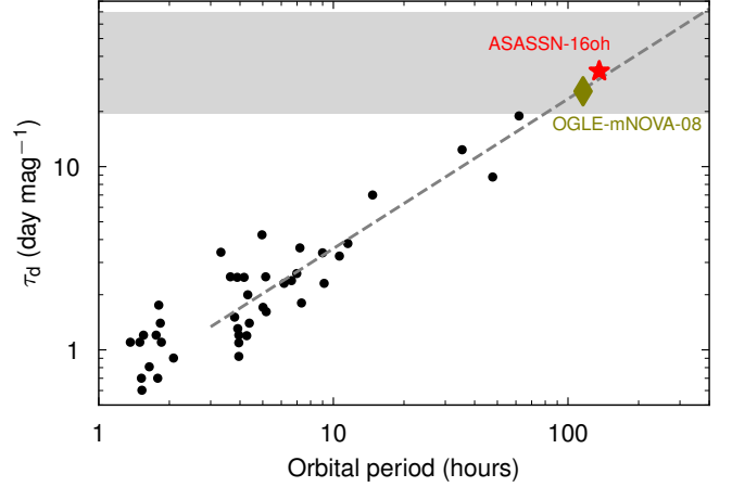
Figure 6. Orbital period ( P_{\text{orb}} )–decline rate ( \tau_d ) relation for dwarf nova outbursts, using data from Simon (2021), and extended to include the range of decline rates (gray area) observed in millinovae ( 20 \lesssim \tau_d \lesssim 70 \text{ day mag}^{-1} ). The red asterisk and green diamond mark the locations of ASASSN-16oh (Rajaelimanana et al. 2017) and OGLE-mNOVA-08, respectively.
