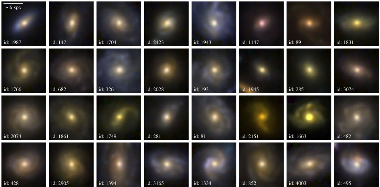
Figure 1. The three colour images ( F150W , F277W , F444W ) of the 32 galaxies used in this work have dimensions of 70 \times 70 pix, or 2.1 \text{ arcsec} \times 2.1 \text{ arcsec} . They are arranged in order of increasing RA and Dec. All are within a redshift range of 1.43 \leq z \leq 1.74 and have stellar masses of 10^{10.5-11.4} M_{\odot} . The FMOS ID for each galaxy is provided in the bottom-left corner, with their corresponding properties listed in Table C1. The F150W and F277W images are PSF-matched to the F444W image using a Gaussian kernel. However, this work does not require PSF matching; it is performed here solely for illustration purposes.
