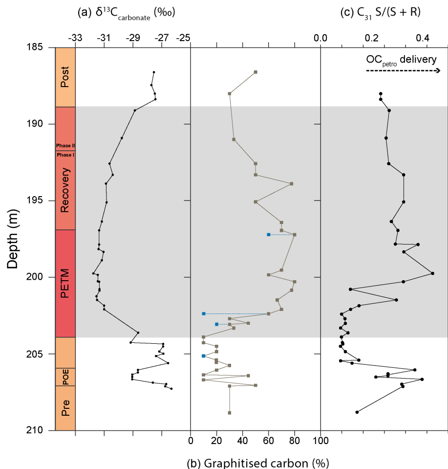
Figure 3 The SDB record of (a) bulk sediment \delta^{13}\text{C}_{\text{carbonate}} ( \delta^{13}\text{C}_{\text{carbonate}} ; Lyons et al. , 2019), (b) percentage graphitised carbon (this study), and (c) \text{C}_{31} homohopane 22S/(22S + 22R) ratio (Lyons et al. , 2019). The blue symbols within panel (b) are the duplicate measurements. The time intervals are as follows: pre-PETM, PETM (onset/body), Recovery Phase I, Recovery Phase II, and post-PETM, based on Hollingsworth et al. (2024) and references therein. The POE in the pre-PETM interval is isolated using the definition from Babila et al. (2022).
