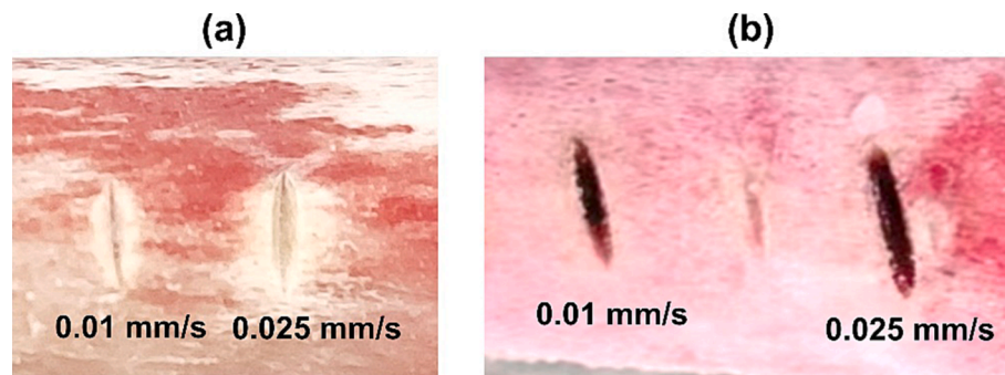
Fig. 19. Ex-vivo chicken femur samples showing the cuts made for the (a) matched hard PZT and (b) Mn:PIN-PMN-PT surgical devices operating at a displacement amplitude of 60 \mu\text{m}_{\text{p-p}} .
