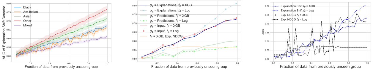
Figure 3: Novel group shift experiment on the US Income dataset. Sensitivity (AUC) increases with the growing fraction of previously unseen social groups. Left figure: The explanation shift indicates that different social groups exhibit varying deviations from the distribution on which the model was trained (White). Middle Figure: We vary the model f_\theta by training it using both XGBoost (solid lines) and Logistic Regression (dots). The novel ethnicity group is Black. We compare Explanation Shift against C2ST on input ( B6 ) and output ( B7 ). Right figure: Comparison of Explanation Shift against Exp. NDCG ( B4 ). We see how monitoring method ( B4 ) is more unstable with a linear model, and with an XGBoost it erroneously finds a horizontal asymptote. We don't compare against methods relying purely on input data such as ( B1 ) as we are changing the model, which they don't take into consideration.
