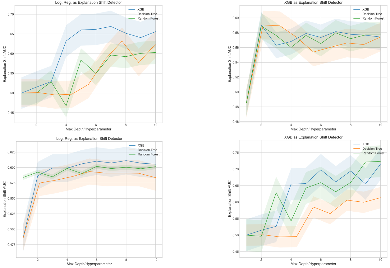
Figure 5: Images represent the AUC of the Explanation Shift Detector , on two dataset: Top ACS Income and Bottom Stackoverflow under novel group shift. In the images on the left, the detector is a logistic regression, and in the images on the right, it is a gradient-boosted decision tree classifier. By changing the model, we can see that vanilla models (decision tree with depth 1 or 2) are unaffected by the distribution shift, while when increasing the model complexity, the out-of-distribution impact of the data in the model starts to be tangible
