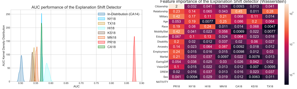
Figure 7: The left figure compares the performance of the Explanation Shift Detector in different states for the ACS Employment dataset. The right figure shows the feature importance analysis for the same dataset.
