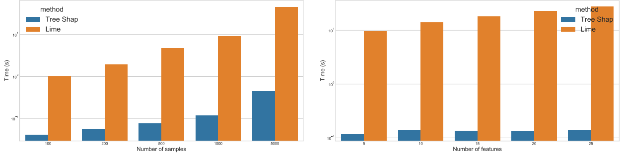
Figure 13: Wall time for generating explanation distributions using SHAP and LIME with different numbers of samples (left) and different numbers of columns (right). Note that the y-scale is logarithmic. The experiments were run on a server with four vCPUs and 32 GB of RAM. The runtime required to create an explanation distribution with LIME is far greater than SHAP for a gradient-boosted decision tree
