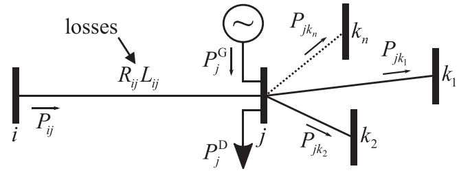
Fig. 2. Graphical representation of the DistFlow branch equations.
