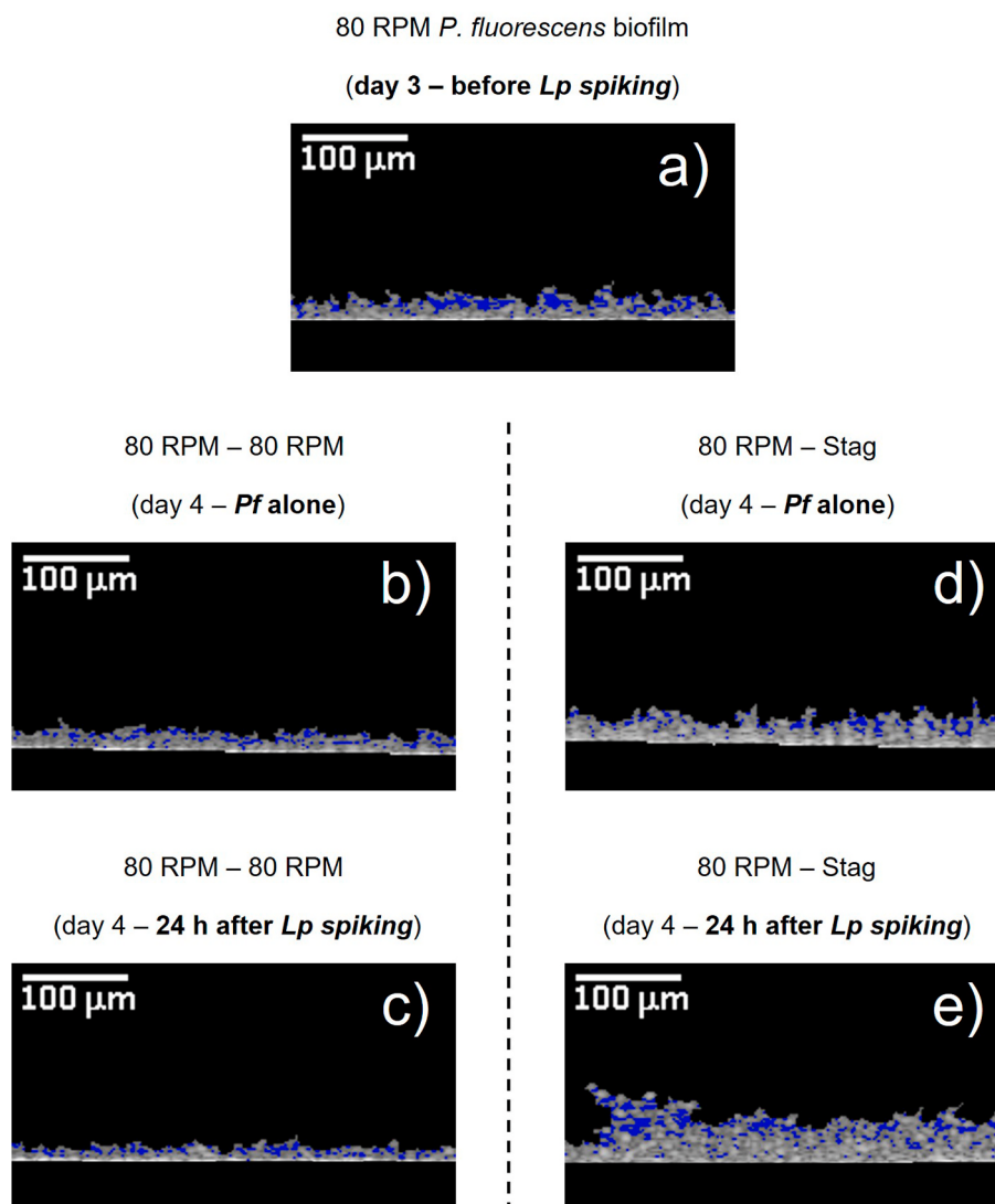
Fig. 2. Representative images obtained by 2D – Optical Coherence Tomography (OCT) of (a) pre-established P. fluorescens ( Pf ) biofilms before L. pneumophila ( Lp ) spiking (on day 3), and Pf biofilms (b) alone on day 4 (control) and (c) 24 h after Lp spiking under 80 RPM (80 RPM – 80 RPM) – left side, and (d) alone on day 4 (control) and (e) 24 h after Lp spiking and reincubation under stagnation (80 RPM – Stag) – right side. The empty spaces within the biofilm structure are coloured blue. (For interpretation of the references to colour in this figure legend, the reader is referred to the Web version of this article.)
