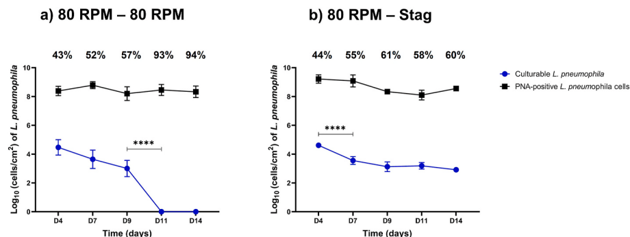
Fig. 7. The number of culturable (CFU, \log_{10} CFU/cm 2 or mL) and PNA-positive cell counts of L. pneumophila (Lp; cells/cm 2 ) over time for (a) 80 RPM – 80 RPM and (b) 80 RPM – Stag biofilms. The percentages of the Lp population in VBNC are shown for each timepoint and were calculated considering the culturable and the total Lp cell counts. The mean \pm standard deviation ( n = 12 for the culturable cells and n = 120 for the PNA-positive cell counts) shown includes three independent experiments with two replicates (coupons) each. Statistically significant differences are represented for p < 0.0005 by *** and < 0.0001 by ****.
