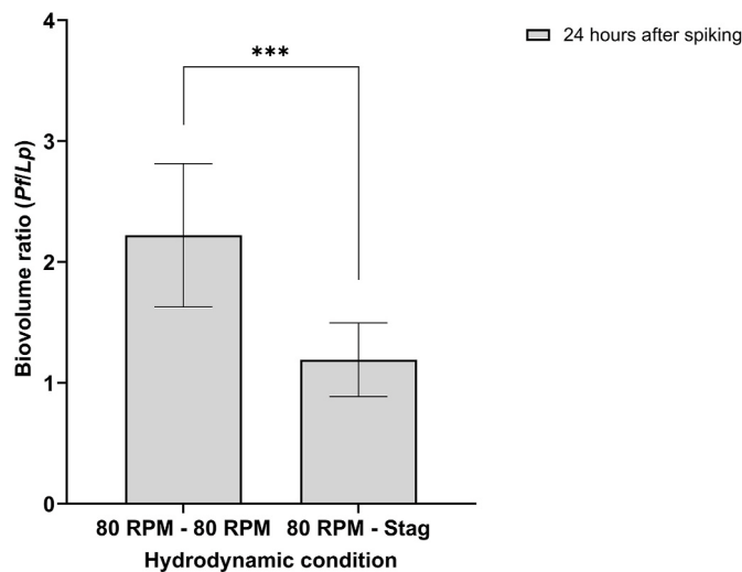
Fig. 6. The ratio of the biovolumes of P. fluorescens (Pf) and L. pneumophila (Lp) in spiked biofilms 24 h after spiking with hydrodynamic conditions set to 80 RPM (80 RPM – 80 RPM) and to stagnation (80 RPM – Stag). The biovolume values were extracted from confocal microscopy images with the COMSTAT plugin. The mean \pm standard deviation ( n = 18 ) shown includes three independent experiments with two replicates (coupons) each. Statistically significant differences are represented for p < 0.0005 by ***.
