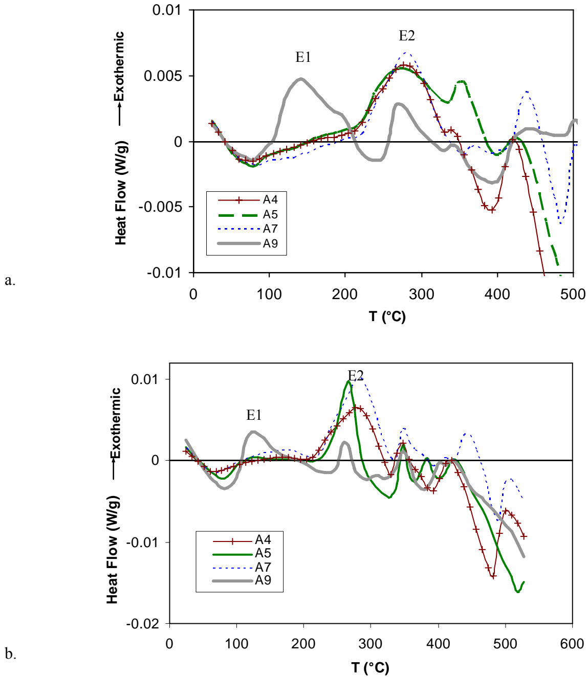
Fig. 9 DSC data for selected Cu-containing alloys solutionised 30 minutes at a) 500°C, b) 550°C
