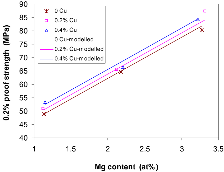
Fig. 6 Measured 0.2% proof strengths of solution treated alloys and their prediction.
