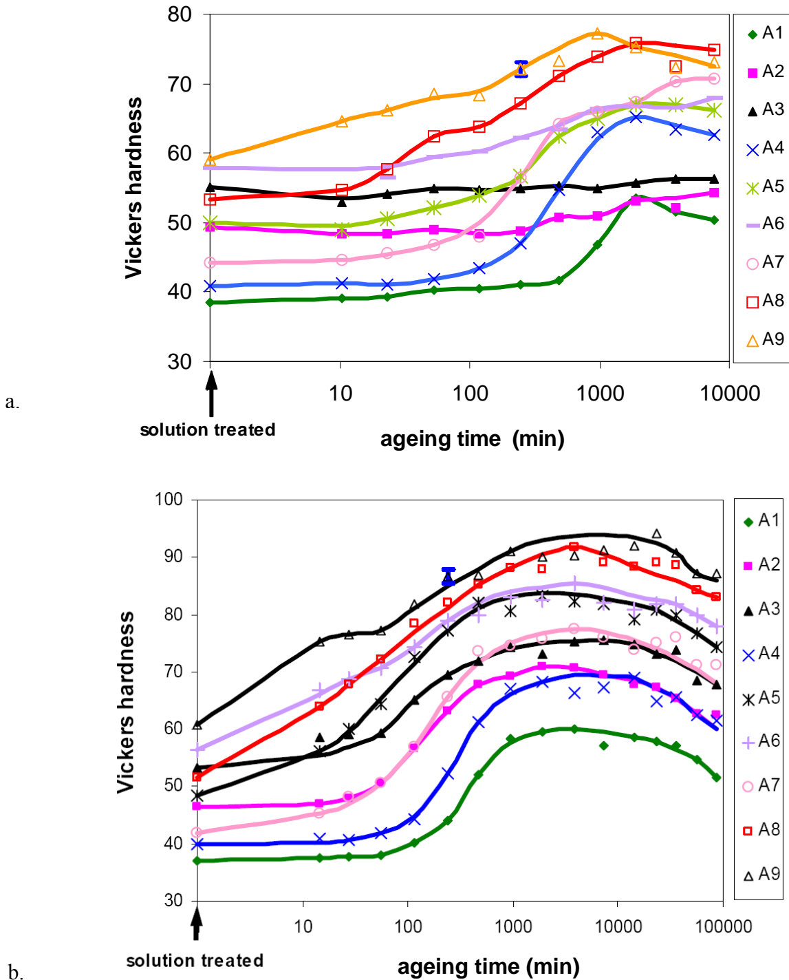
Fig. 7 Hardness during isothermal ageing at 170°C for solution treated samples solutionised 30 minutes at a) 500°, and b) 550°C. In each graph, one error bar is shown, which indicates the average of the standard deviations of all tests reported in that graph.
