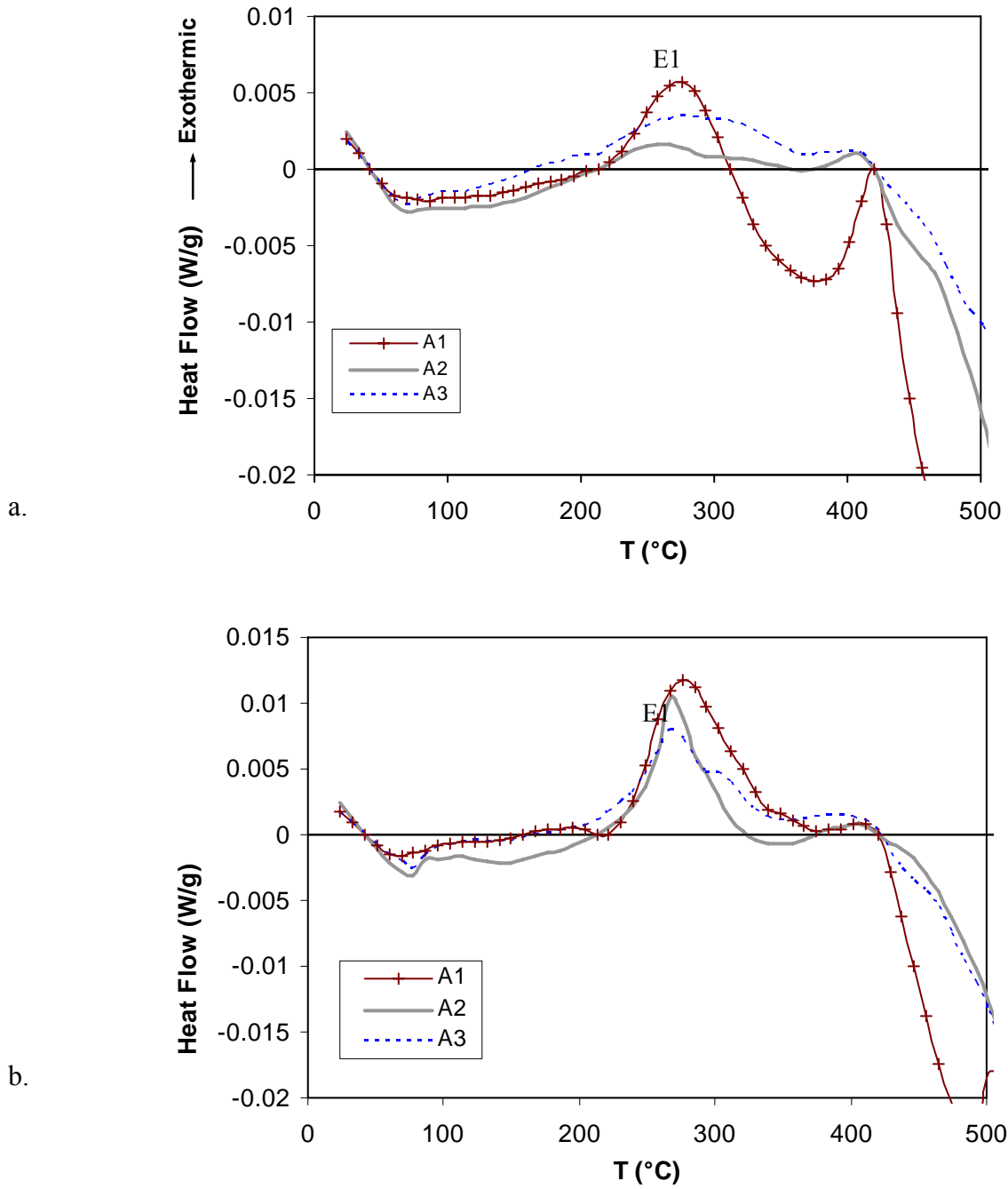
Fig.8 DSC data for Cu-free alloys solutionised 30 minutes at a) 500°C, b) 550°C
