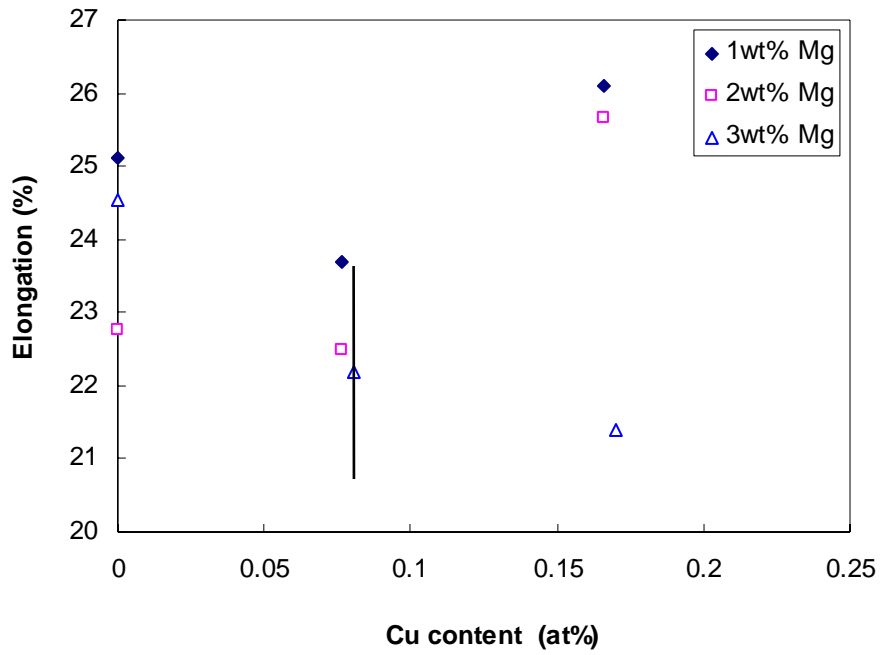
Fig. 4 Tensile test data vs. Cu contents for solution treated samples: a. 0.2% proof strength, b. UTS, c. elongation. Bars on one point represent the average spread in measured values for each data point.
