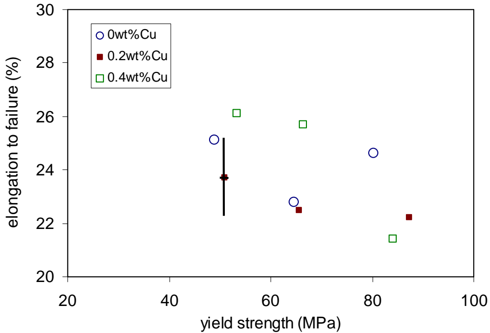
Fig. 5 Elongation to failure vs tensile yield strength for the 9 alloys in solution treated condition. Bars on one point represent the average spread in measured values for each data point.
