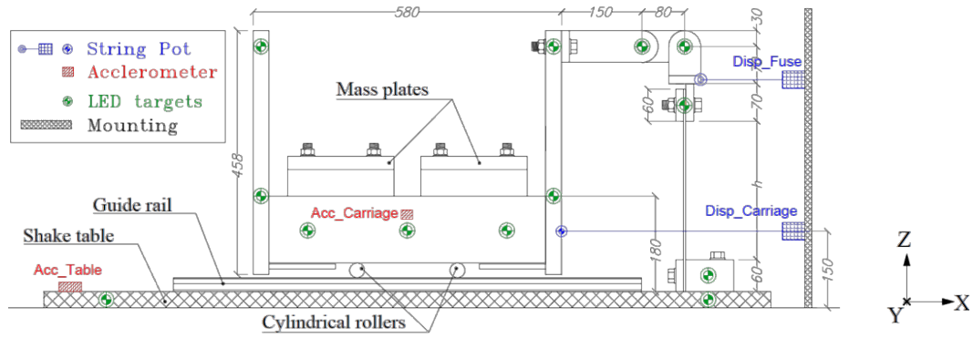
Fig. 4 Instrumentation layout
