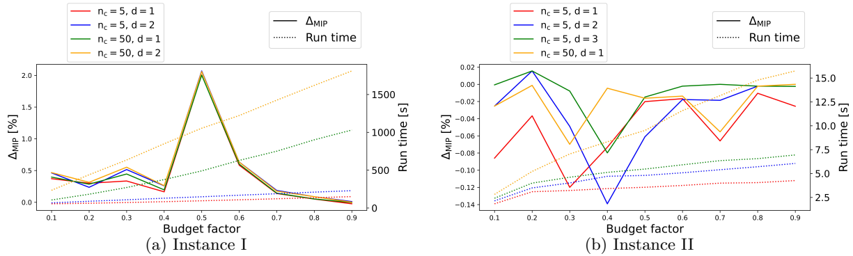
Figure 3 Performance of the open greedy algorithm for choices of n_c and d . The initial and final assignment methods are m = \text{greedy assign with local search reassign} and m' = \text{relaxation rounding with local search reassign} , respectively. We use n_r = 50 . For details, see Section 6.3.2.
