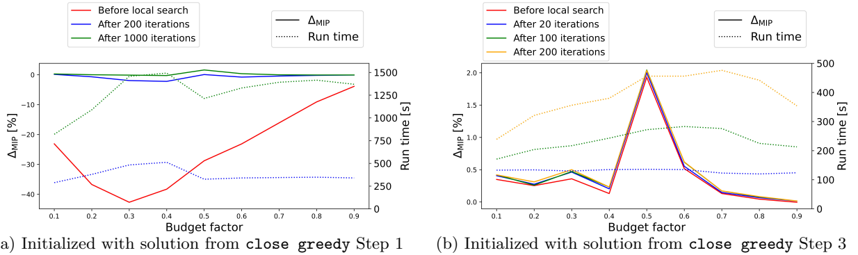
Figure 4 Performance of the BFLP local search with n_c = 50, d = 2 on Instance I. The final assignment method is m' = \text{relaxation rounding with local search reassign} . We use n_r = 50 . These run times are for the local search alone. For details, see Section 6.3.3
