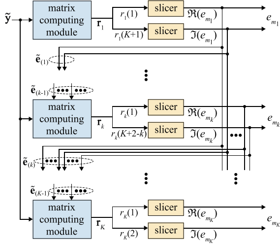
Fig. 1. Structure of the proposed memristor-based SIC detector circuit.
