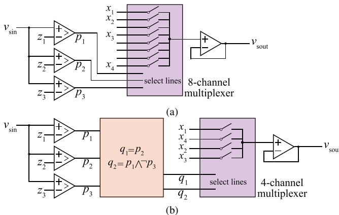
Fig. 4. The proposed slicer with: (a) the directly select structure, and (b) the indirectly select structure, using 16 QAM as an example.
