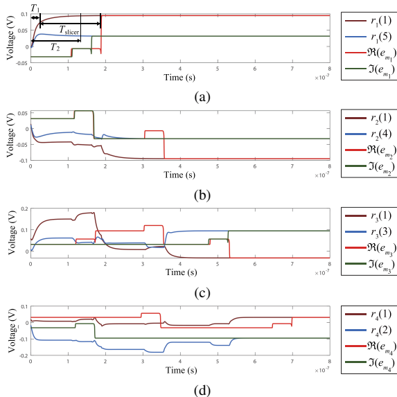
Fig. 6. Voltage waveforms at input and output nodes of slicers in the four stages of the proposed circuit: (a) the first stage, (b) the second stage, (c) the third stage, (d) the fourth stage.
