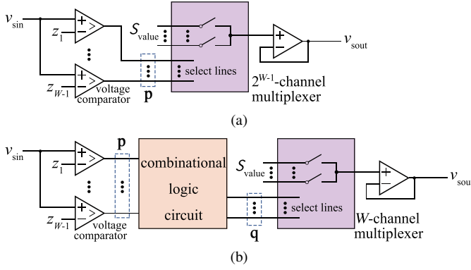
Fig. 3. Structures of the proposed slicer: (a) the directly select structure, and (b) the indirectly select structure.
