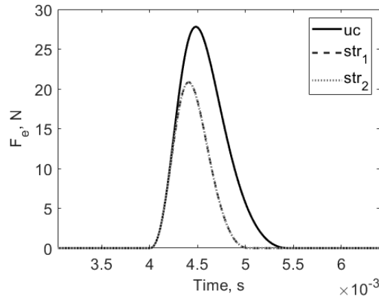
Figure 3. Hammer-string contact force. uc: una corda . str1: string one (nominal tension) in normal playing conditions. str2: string two (with tension modification) in normal playing conditions
