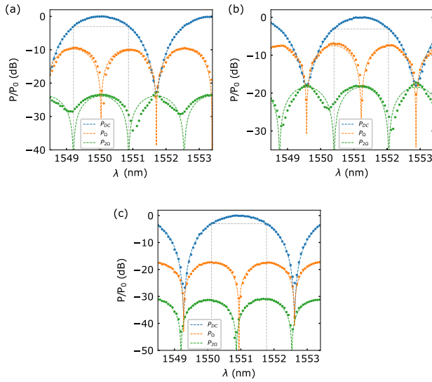
Fig. 7. Measurements (dots) of P_{DC} , the MZM output DC optical power; P_{\Omega} , the modulation at angular frequency \Omega ; P_{2\Omega} , the modulation at angular frequency 2\Omega as a function of wavelength for (a) the 2 mm long PN junction using V_{DC} = 2 V, V_{RF} = 0.51 V, (b) the 5 mm long PIN2 junction using V_{DC} = 4 V, V_{RF} = 1.6 V, and (c) the 5 mm long PIN3 junction using V_{DC} = 6 V, V_{RF} = 2.0 V. The dashed lines represent the corresponding fit.
