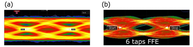
Fig. 5. Optical eye diagram display from 1 mm long PIN3 modulator by applying dual 2V_{\text{pp}} DATA/ \overline{\text{DATA}} driving in push-pull and reverse V_{\text{DC}} = 30 V measured at (a) 80 Gbit/s and (b) 100 Gbit/s with a numerical six taps feed-forward equalization (FFE).
