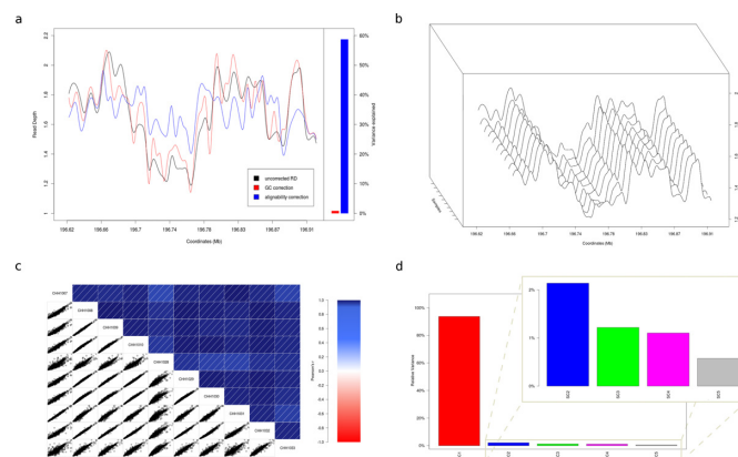
Figure 1. Read depth profiles. (a) Read depth profile of sample CHH1030 (RCA cohort) across the target region, before and after correcting for GC-content and alignability using linear regression. The coefficient of determination ( R^2 , ratio of explained variation to the total variation) is used to determine the variance explained by each variable. GC explains only a small fraction of the read depth variance, while alignability explains 57%. (b) Read depth profile for 10 randomly chosen samples from the RCA cohort across the target region. The profiles appear to have a high degree of similarity, with only minor variations between samples. (c) Correlogram for the 10 samples in (b). The lower left panel represents the pair-wise scatterplot for all possible sample combinations. The upper right panel represents the color- and intensity-coded Pearson's correlation ( r^2 ) for all possible sample combinations. The minimum reported r^2 is 0.93. (d) The relative variance for the first five singular components calculated from our entire dataset. The relative variance of component k is defined as s_k^2 / \sum_i s_i^2 . The first singular component dominates with a relative variance of 93%, while the remaining components have minor contributions.
