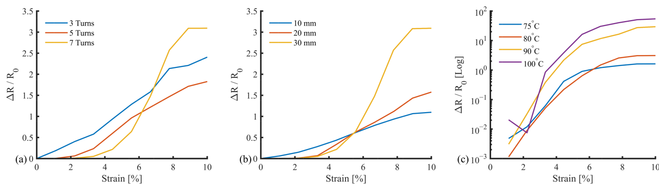
Figure 7. Sensor parameterisation: (a) Turns: three, five, and seven, (b) Lengths: 10 mm, 20 mm, 30 mm, and (c) Cure temperature 75 °C, 80 °C, 90 °C, and 100 °C.
