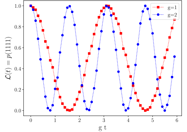
FIG. 2. Oscillations of the Loschmidt probability \mathcal{L}(t) = p(1111) for the square \mathbb{Z}_2 plaquette on the ibmq_qasm_simulator, which is a general-purpose simulator. The points are the points from the simulator, and the line is provided only to guide the eye. The system has a two-dimensional gauge-invariant Hilbert space, and there is a two-state Rabi oscillation when started from the state |1111\rangle to the state |0000\rangle . An identical behavior is also observed in the triangular \mathbb{Z}(2) plaquette. Increasing the coupling by a factor of 2 is identical to speeding up the dynamics by a factor of 2.
