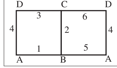
FIG. 4. The setup for two plaquettes which have periodic boundary conditions in the longer direction. The links are marked with numerals, while the sites are marked with letters.
