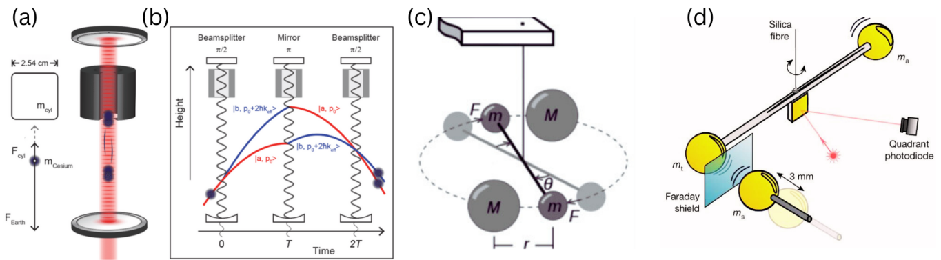
FIG. 9 Experimental setup and interferometry measurement. (a) Setup for measuring Cesium atoms' acceleration towards a 0.19 kg tungsten cylinder in ultrahigh vacuum. The cylinder is 2.54 cm in height and diameter, with a 0.5 cm axial through-hole and slot width. Differential measurements are used to study interactions with the mass. (b) A Mach-Zehnder interferometer using Raman transitions in an optical cavity. Three laser pulses manipulate Cesium atoms, splitting, reflecting, and recombining them to measure phase differences, providing an ensemble-averaged acceleration over 110 ms across approximately 100,000 atoms. Adapted from (Jaffe et al. , 2017). (c) Schematic of a Cavendish torsion balance with dumbbell masses ( M ), external forces ( F ), and resulting rotation angle ( \theta ). (d) Torsion pendulum as a gravitational acceleration transducer, containing two gold spheres (1 mm radius, 40 mm apart) on a glass capillary. One sphere serves as a test mass (90.7 mg), the other as a counterbalance (91.5 mg). A silica fiber with a diameter of 4 \mu\text{m} supports the pendulum with a 3.6 mHz torsional resonance. The torsion angle is detected optically. The source mass (92.1 mg) is harmonically moved 3 mm at 12.7 mHz to enhance the gravitational signal. Electrostatic interference is reduced using Faraday shield and discharging techniques. Adapted from (Westphal et al. , 2021).
