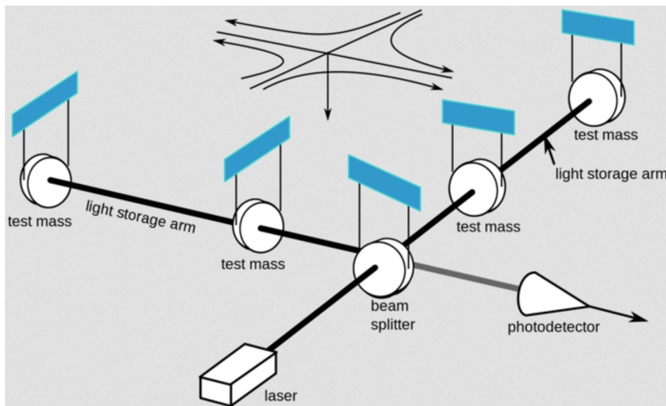
FIG. 10 LIGO laser interferometer setup. The interference of light in the two arms leads to the detection of extremely small displacements. Adapted from (Scharpf et al. , 2017).
