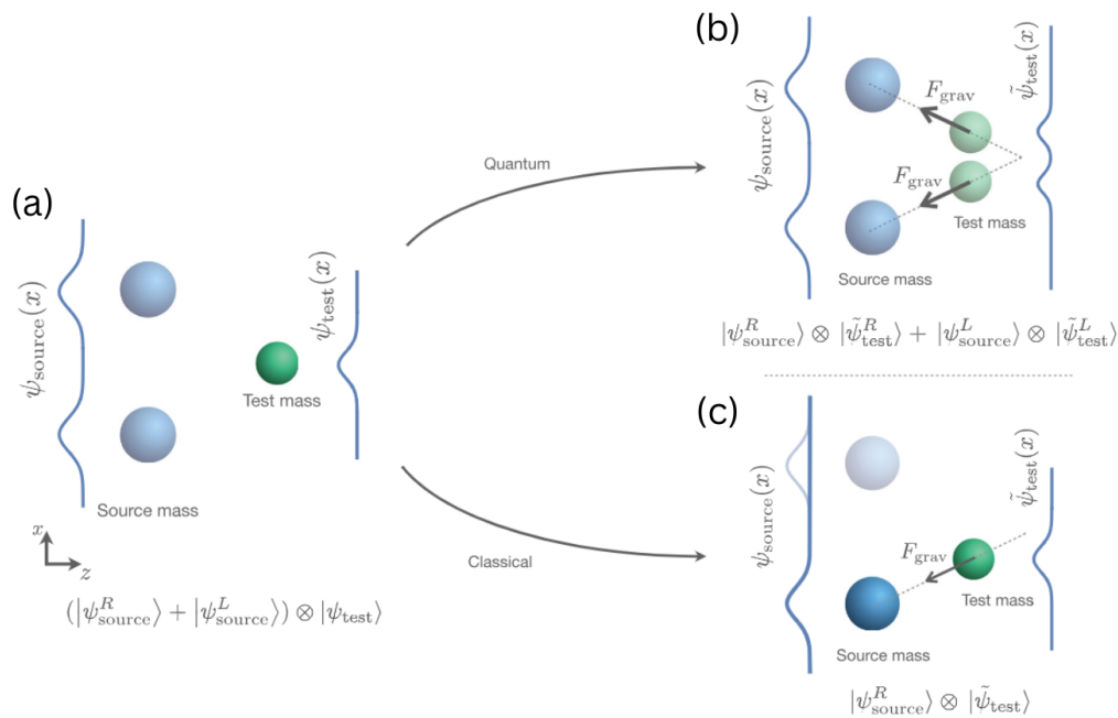
FIG. 11 Feynman’s thought experiment. (a) A gravitational field source (blue ball) is placed in a quantum superposition and interacts with a test mass (green ball). The system can develop into two scenarios: (b) If the field is in a quantum superposition, the test mass feels two different gravitational forces and also enters a superposition state. (c) If the field stays classical, the test mass feels a single gravitational force and moves accordingly. Adapted from (Pedernales and Plenio, 2023).
