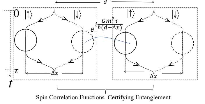
FIG. 4 Mechanism of gravitationally generated entanglement. Mechanism of entanglement of two masses through the phase evolution due to gravitational interaction. The phase evolution due to only the most prominent interaction, between the |R \downarrow\rangle_1 and |L \uparrow\rangle_2 is explicitly shown. The figure is a modified version of (Bose et al. , 2017).
