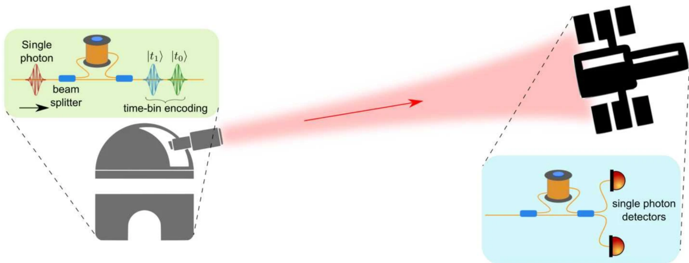
FIG. 8 Simplified diagram of the optical COW experiment in space. A single photon is split into two paths using an unbalanced Mach-Zehnder interferometer (MZI). This photon is then transmitted to a satellite with an identical MZI. The interference observed at the satellite shows the phase shift caused by gravity. Adapted from (Mohageg et al. , 2022).
