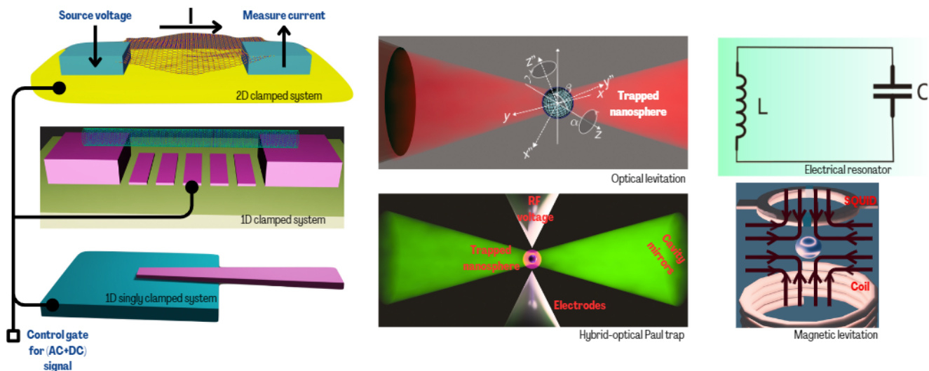
FIG. 5 Illustration of state-of-the-art mechanical systems. This figure encapsulates an array of resonators utilized in experimental efforts aimed at detecting the interplay between quantum mechanics and gravity. The leftmost column showcases mechanical resonators: a 2D clamped resonator (Graphene), a 1D clamped resonator (A suspended carbon nanotube), and a 1D singly clamped beam resonator, illustrating the diversity in mechanical systems. The central column depicts optical levitation systems: a standalone optical levitation and a hybrid Paul-optical levitation system, demonstrating the integration of optical techniques. The rightmost column presents an electrical resonator and a magnetic levitation system, representing the incorporation of electromagnetic methodologies. Together, these systems exemplify the wide range of experimental apparatuses employed in the quest to uncover the interplay between quantum mechanics and gravity.
