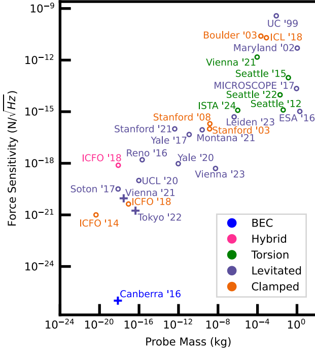
FIG. 7 Force sensitivities achieved with massive probe systems. The colors correspond to BECs (blue), hybrid systems (pink), torsion balances (green), levitated systems (purple), and clamped systems (orange). Plus signs indicate that the system contains less than one thermal phonon. We classify systems as hybrid whenever a qubit or similar system is used to interface with the mechanical element. The data points correspond to the following references: Canberra '16: (Hardman et al. , 2016), Boulder '03: (Long et al. , 2003), Stanford '03: (Chiaverini et al. , 2003), Stanford '08: (Geraci et al. , 2008), ICL '18: (Pike et al. , 2018), ICFO '18: (De Bonis et al. , 2018), ICFO '14: (Moser et al. , 2014), ICFO '18: (Tavernarakis et al. , 2018), UC '99: (Goodkind, 1999), Maryland '02: (Moody et al. , 2002), Reno '16: (Ranjit et al. , 2016), Soton '17: (Hempston et al. , 2017), Yale '17: (Monteiro et al. , 2017), Yale '20: (Monteiro et al. , 2020), UCL '20: (Pontin et al. , 2020), Montana '21: (Lewandowski et al. , 2021), Vienna '21: (Magrini et al. , 2021), Stanford '21: (Blakemore et al. , 2021), Tokyo '22: (Kamba et al. , 2022), Leiden '23: (Fuchs et al. , 2023), Vienna '23: (Hofer et al. , 2023), ESA '16: (Armano et al. , 2016), MICROSCOPE '17: (Touboul et al. , 2017), Seattle '12: (Wagner et al. , 2012), Seattle '15: (Terrano et al. , 2015), Vienna '21: (Westphal et al. , 2021), Seattle '22: (Shaw et al. , 2022), ISTA '24: (Agafonova et al. , 2024).
