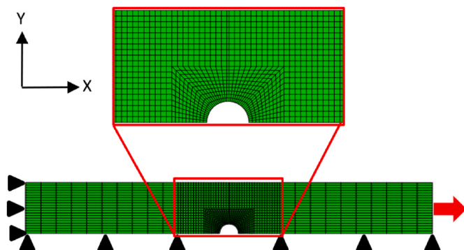
Fig. 5. Mesh and boundary conditions.
