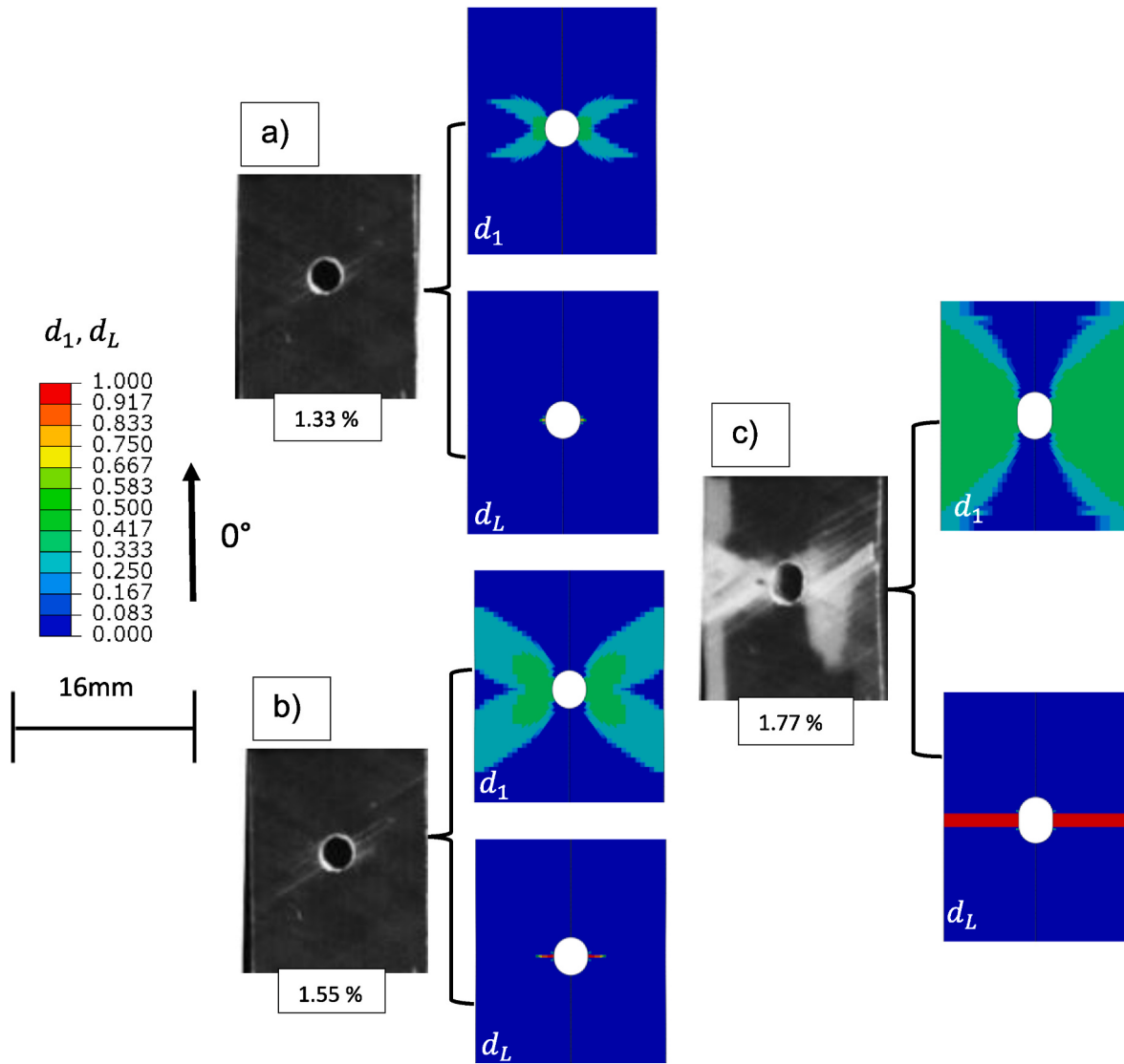
Fig. 9. Damage development of the specimen at different strains in experimental and numerical results evaluating the damage progress ( d_1 ) and crack progress ( d_L ) for \pm 60\text{QI}/\text{Hexcel} . Experimental pictures are adapted from (Fotouhi et al., 2018).
