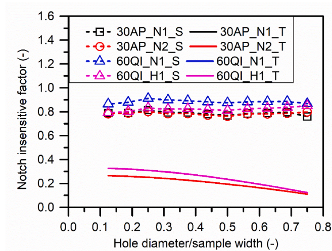
Fig. 10. Simulation (S) and theoretical (T) notch insensitive factors for different hybrid configurations and hole diameter/sample width ratios.
