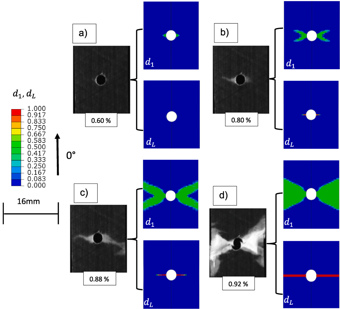
Fig. 8. Damage development of the specimen at different strains in experimental and numerical results evaluating the damage progress ( d_1 ) and crack progress ( d_L ) for \pm 60^\circ QI/North. Experimental pictures are adapted from (Fotouhi et al., 2018).
