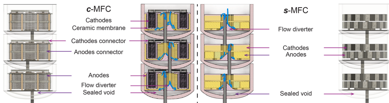
Fig. 1. Cross section view of the ceramic-based ( c -MFC; left) and the membrane-less MFC ( s -MFC; right) cascades used in this study.
