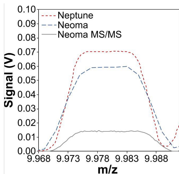
Figure 7. Mass scan from m/z of 9.968 to 9.992 showing the ^{40}\text{Ar}+\text{Ca}^{4+} peak when ablating NIST SRM612 or JCp-1 (transect mode, 100 \mu\text{m} diameter laser beam, 6 J \text{cm}^{-2} laser energy density, 12 Hz repetition rate, 10 \mu\text{m s}^{-1} tracking speed) on a Neptune MC-ICP mass spectrometer (dashed red line), a Neoma MC-ICP mass spectrometer (dashed blue line), and a Neoma MS/MS MC-ICP mass spectrometer (solid grey line). Note that normalising to sensitivity does not impact the overall picture.
