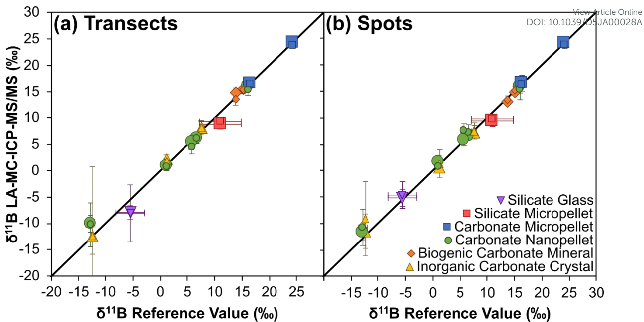
Figure 2. Mean LA-MC-ICP-MS/MS \delta^{11}\text{B} ( \pm 2\text{SD} ) versus reference value \delta^{11}\text{B} (Table 1) for the 14 reference materials analysed in this study: (a) transect measurements, (b) spot measurements. Data label size correlates to laser beam size: smaller labels correspond to either 50 by 50 \mu\text{m} square (transect) or 50 \mu\text{m} diameter circle (spot) laser beams, and larger labels correspond to 80 by 80 \mu\text{m} square (transect) or 80 \mu\text{m} diameter circle (spot) laser beams. Solid black line represents 1:1 ratio.
