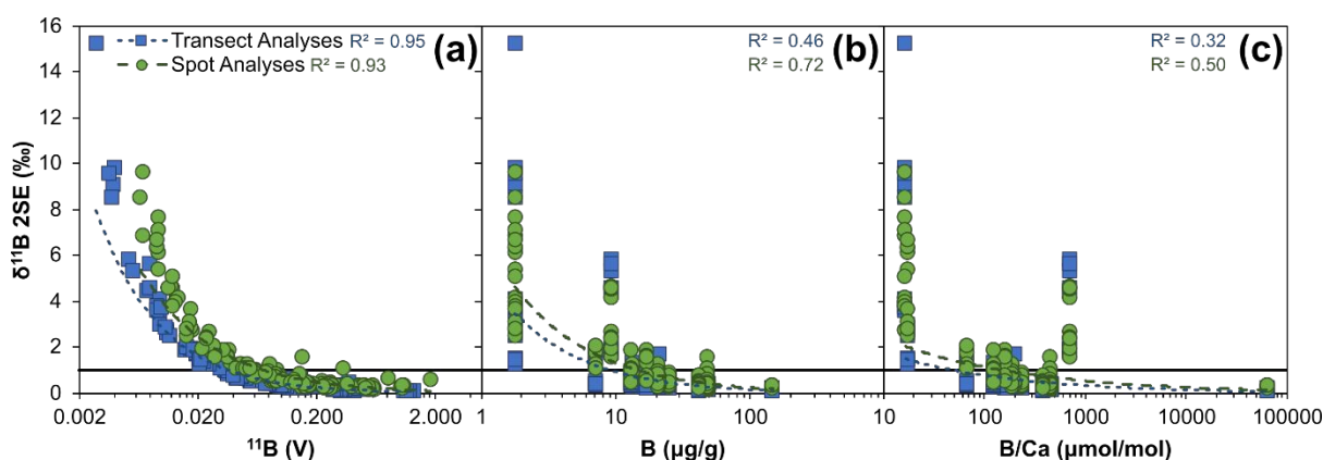
Figure 4. Boron isotope internal precision (2SE) of 14 reference materials analysed by LA-MC-ICP-MS/MS: (a) plotted against ^{11}\text{B} signal (V), (b) plotted against boron \mu\text{g/g} , and (c) plotted against B/Ca ( \mu\text{mol/mol} ). Solid black line represents 2SE of 1 ‰. Dashed coloured lines show power relationship of all transect or spot data respectively, with R^2 included.
