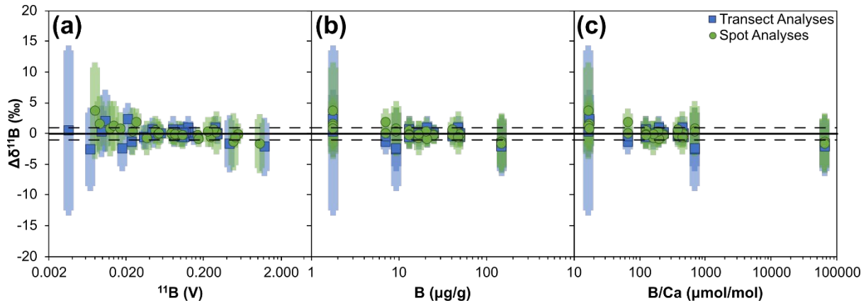
Figure 3. Boron isotope accuracy ( \Delta\delta^{11}\text{B} ) of 14 reference materials analysed by LA-MC-ICP-MS/MS: (a) plotted against ^{11}\text{B} signal (V), (b) plotted against boron \mu\text{g/g} , and (c) plotted against B/Ca ( \mu\text{mol/mol} ). Solid horizontal bar represents \Delta\delta^{11}\text{B} of 0 ‰, dashed horizontal bar represents \Delta\delta^{11}\text{B} of +1 ‰ and -1 ‰ respectively. Uncertainties are the 2SD of the repeat measurements by LA-MC-ICP-MS/MS summed in quadrature with the uncertainties of the reference values presented in Table 1.
