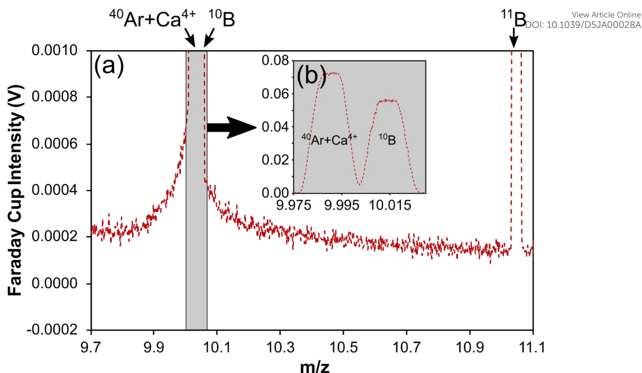
Figure 1. (a) Mass scan across the boron isotope mass range when ablating carbonate reference material collected on a Neptune MC-ICP mass spectrometer, 24 showing the elevated baseline across the entire boron mass range that acts as an interference and impacts the accuracy of boron isotope measurements by LA-MC-ICP-MS. (b) a mass scan showing the well-resolved ^{40}\text{Ar}+\text{Ca}^{4+} and ^{10}\text{B} peaks.
