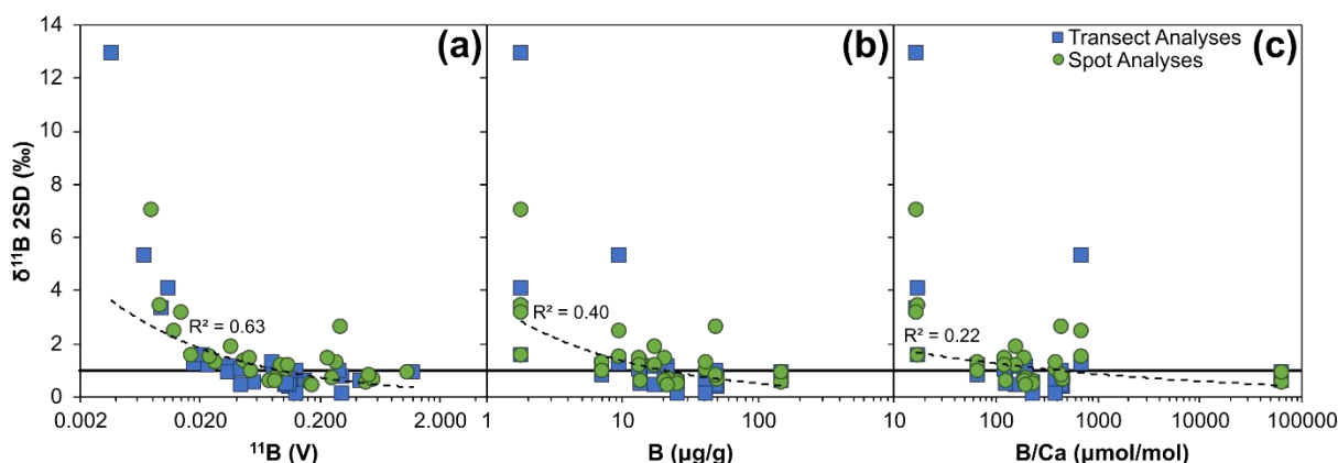
Figure 5. Boron isotope external reproducibility (2SD) of 14 reference materials analysed by LA-MC-ICP-MS/MS: (a) plotted against ^{11}\text{B} signal (V), (b) plotted against boron \mu\text{g/g} , and (c) plotted against B/Ca ( \mu\text{mol/mol} ). Solid black line represents 2SD of 1 ‰. Dashed black line shows power relationship of all data, with R^2 included.
