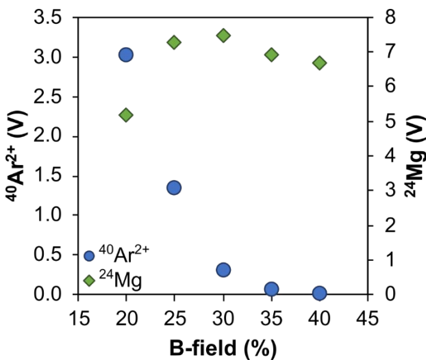
Figure 8. Intensity of ^{40}\text{Ar}^{2+} and ^{24}\text{Mg} beams when a 100 ppb Mg solution is analysed on a Neoma MS/MS MC-ICP mass spectrometer with varying pre-cell mass filter B-fields. Data are available in Supplementary Table S7.
