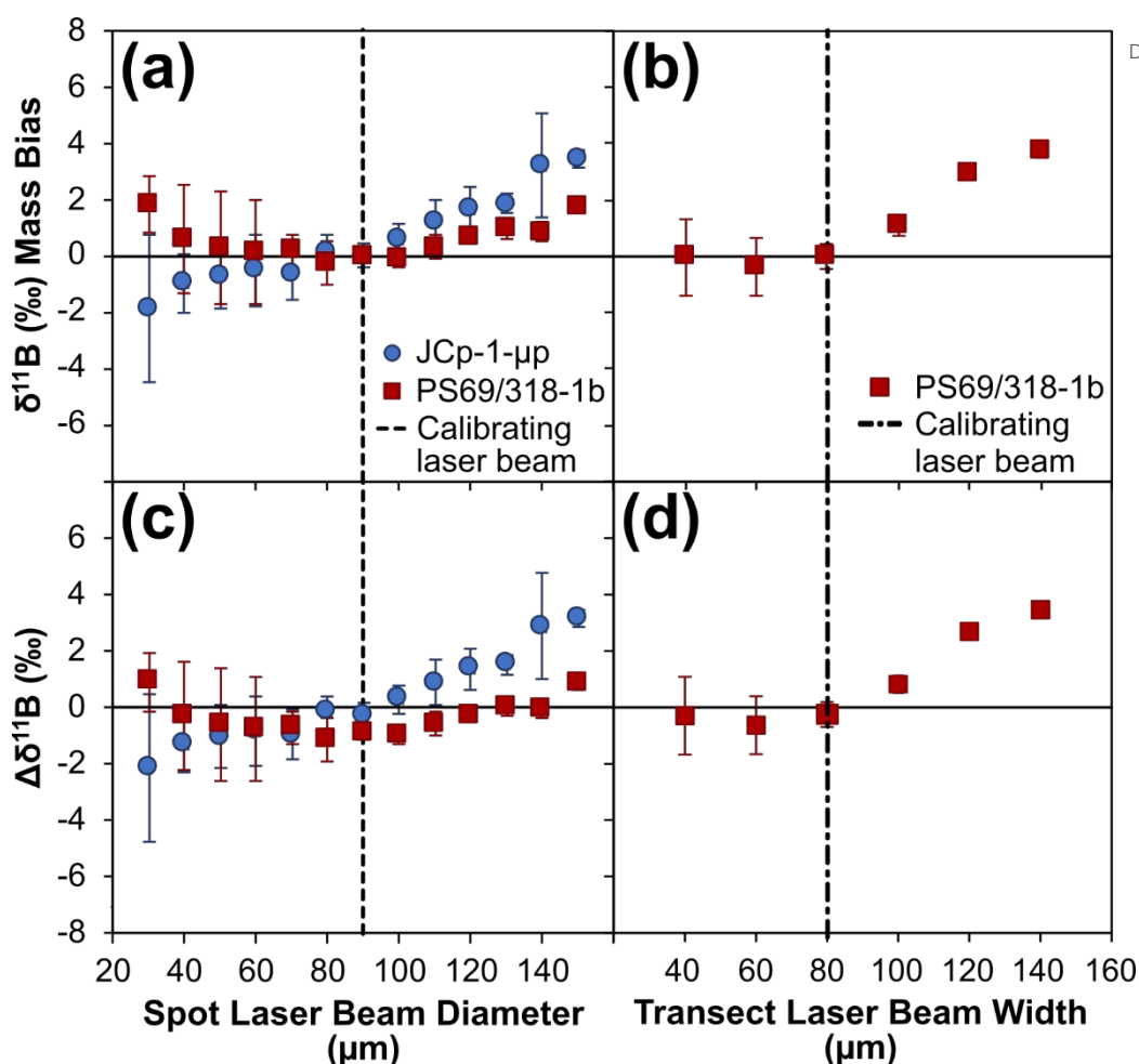
Figure 9. Boron isotope inaccuracy when measuring carbonate reference materials JCp-1 (pressed micropellet) and PS69/318-1b (calcitic coral fragment) under different plasma mass-loading scenarios, following normalisation to NIST SRM612. (a) and (b) expressed as mass bias, calculated by subtracting the measured \delta^{11}\text{B} of the carbonate reference material when analysed using the same sized laser beam to that of the bracketing NIST SRM612 analyses, from the measured \delta^{11}\text{B} of the carbonate reference material when analysed using other laser beam diameters. (c) and (d) expressed as \Delta\delta^{11}\text{B} , calculated by subtracting the \delta^{11}\text{B} reference value of the carbonate reference material in question from the measured \delta^{11}\text{B} . Spot data (a and c) represent the mean of three repeat measurements ( \pm 2\text{SE} ), transect data (b and d) represent single measurements ( \pm 2\text{SE} ). Data are available in Supplementary Table S8.
