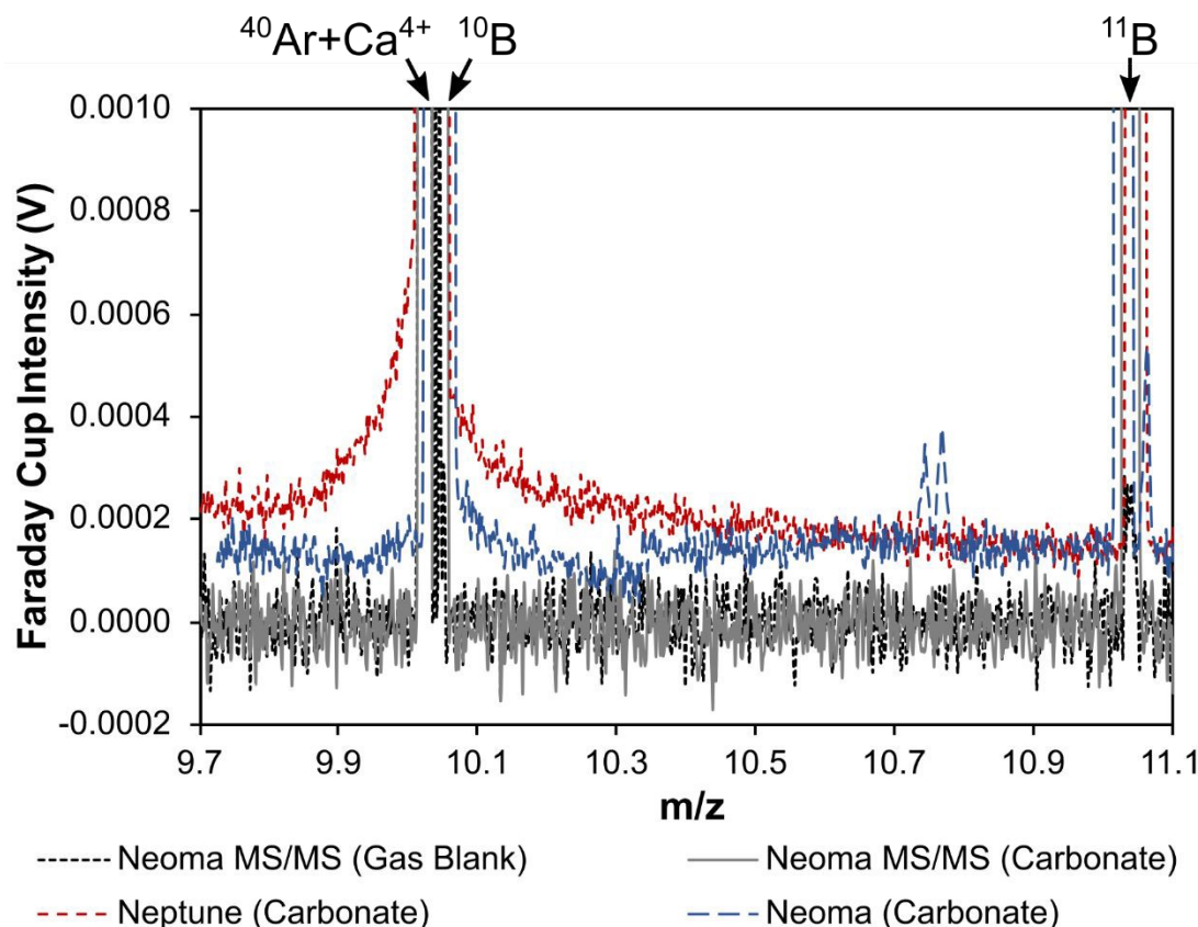
Figure 6. Mass scans across the boron isotope mass range when ablating carbonate reference material collected on a Neptune MC-ICP mass spectrometer, 24 Neoma MC-ICP mass spectrometer, and Neoma MS/MS MC-ICP mass spectrometer. A gas blank mass scan is also shown for the Neoma MS/MS MC-ICP mass spectrometer. Data from the scans are provided in Supplementary Table S6.
