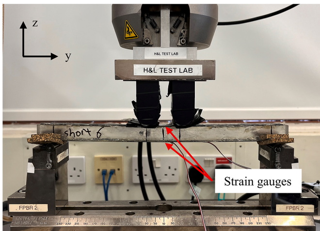
Fig. 4. Experimental setup for the SBB testing (short SBB configuration shown).
