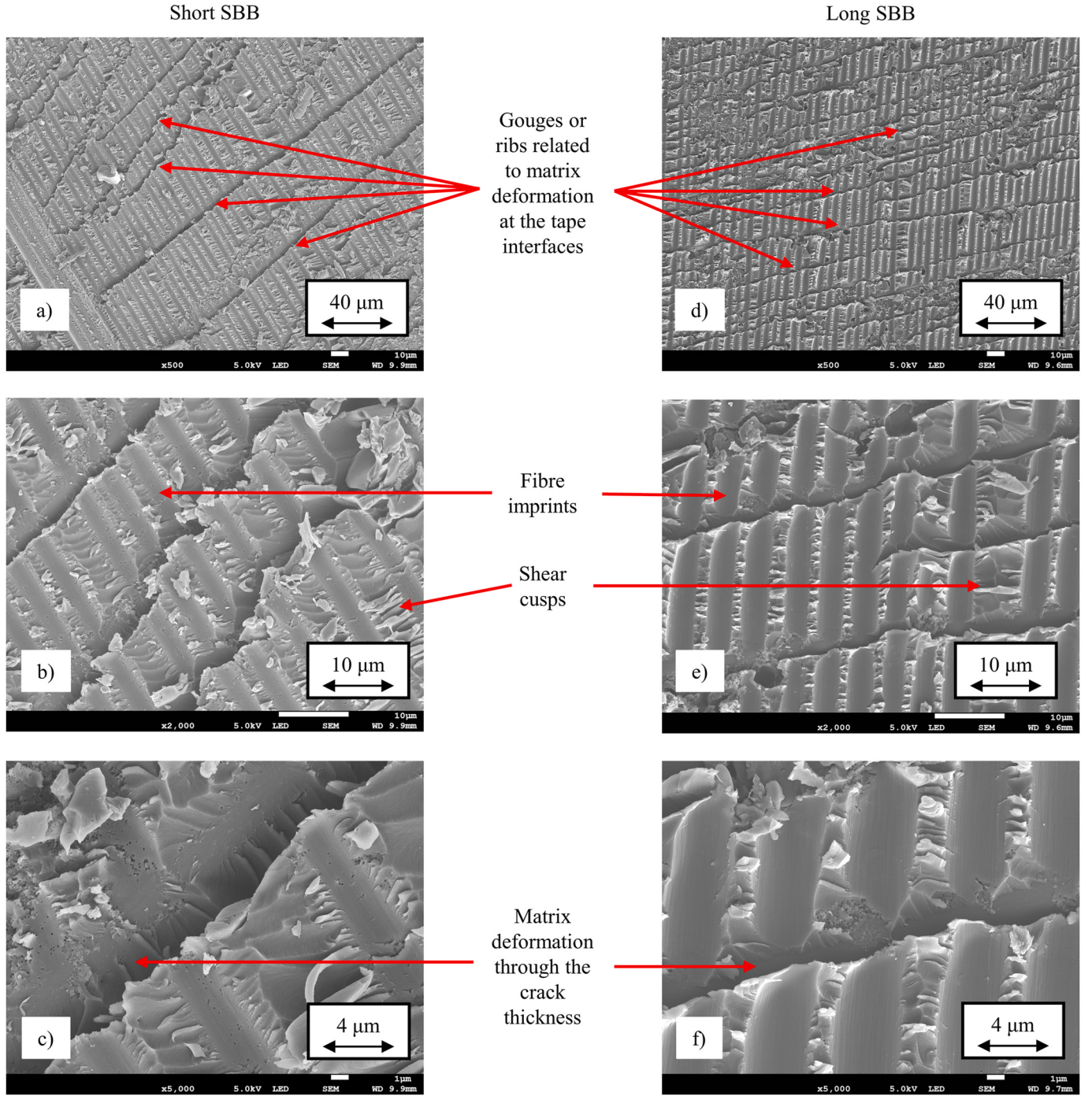
Fig. 10. SEM analysis on the TBDC top skin of the SBB specimen across different scales (x500, ×2000 and ×5000 magnification). The left side shows the short SBB fracture surfaces while the right side shows the long SBB fracture surfaces.
