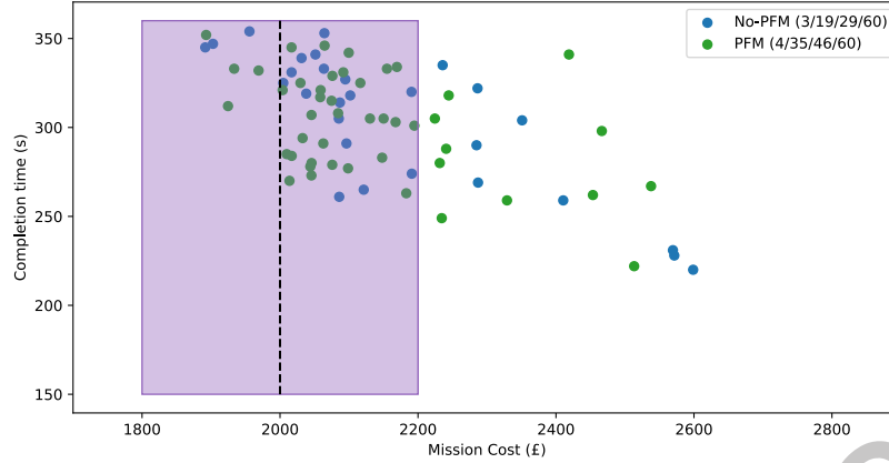
Fig. 4. Plot of mission cost against completion time showing £2000 cost line and its 10% bounded region from £1800 - £2200 for all completed PFM and No-PFM conditions in Experiment 1. The legend shows the number of completions within £2000, the bounded region completions, the total number of completions within time, and the total number of participants in each condition.
