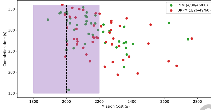
Fig. 8. Plot of mission cost against completion time showing £2000 cost line and its 10% bounded region from £1800 - £2200 for all completed PFM and BRPM conditions in Experiment 2B. The legend shows the number of completions within £2000, the bounded region completions, the total number of completions within time, and the total number of participants in each condition.
