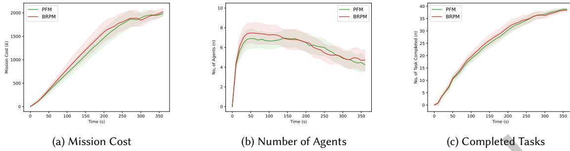
Fig. 7. Comparing the mean performance over time for Experiment 2B. The shaded region around the mean shows the standard deviation.
