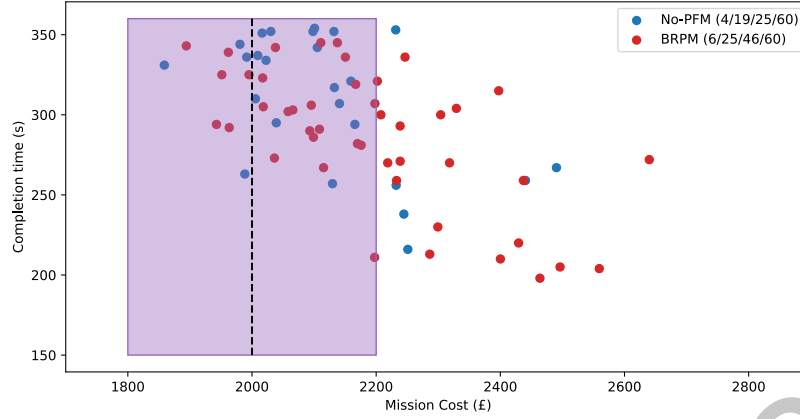
Fig. 6. Plot of mission cost against completion time showing £2000 cost line and its 10% bounded region from £1800 - £2200 for all completed No-PFM and BRPM conditions in Experiment 2A. The legend shows the number of completions within £2000, the bounded region completions, the total number of completions within time, and the total number of participants in each condition.
