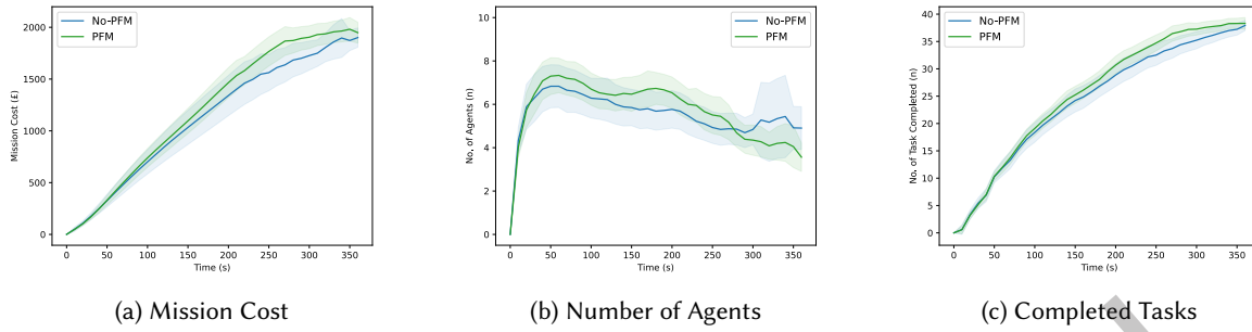
Fig. 3. Comparing the mean performance over time for Experiment 1. The shaded region around the mean shows the standard deviation.
