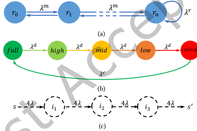
Fig. 1. Partial CTMC: (a) the UAV movement is modelled as transitions between regions r_n , where n \in [0, 8] and r_0 is the hub, with corresponding movement rates \lambda^m and the rotation rate \lambda^r ; (b) the battery drainage is synchronised with draining rates \lambda^d outside the hub and the charging rate \lambda^c in the hub; (c) for each transition s \xrightarrow{\lambda} s' in (a) and (b), intermediate states i_{1 \rightarrow k-1} are introduced to implement the Erlang-k law with transition rates k \cdot \lambda . In this case, we use k = 4 .
