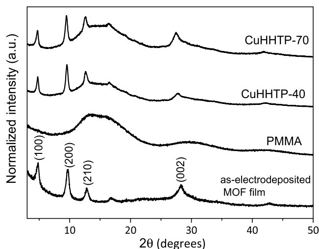
Figure 2. GIXRD patterns of pristine electrodeposited \text{Cu}_3(\text{HHTP})_2 on \text{SiO}_2 , neat PMMA support, and PMMA-transferred \text{Cu}_3(\text{HHTP})_2 thin films dried at 40 ^\circ\text{C} (CuHHTP-40) and 70 ^\circ\text{C} (CuHHTP-70).
