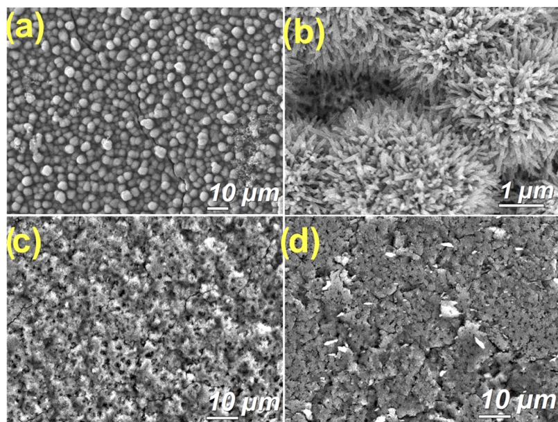
Figure 3. SEM images of as-electrodeposited Cu 3 (HHTP) 2 (a, b) and transferred MOF films dried at 40 °C (c) and 70 °C (d).
