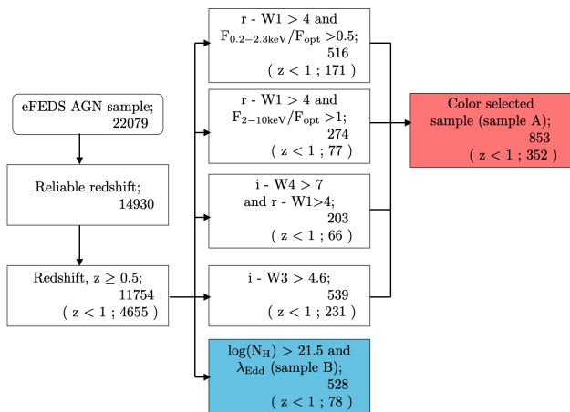
Fig. 3: Flow chart summarising our selection criteria used to isolate candidates from the eFEDS AGN sample. Each box contains a selection method with the cuts applied and the number of sources obtained in the bottom right corner of each box. In brackets, we indicate the number of sources for z less than one ( 0.5 < z < 1 ) which we apply later on for SDSS spectra analysis. By reliable spectroscopic or photometric redshift, we only consider redshift grade 4 or 5 – see Salvato et al. 2022 . F_{\text{opt}} refers to flux in the optical r-band. The box highlighted in red is sample A obtained after applying the colour selections in the top right of Fig. 1. The box highlighted in blue is the N_{\text{H}} > 10^{21.5} \text{ cm}^{-2} and \lambda_{\text{Edd}} > \lambda_{\text{eff}}^{\text{limit}} selection or sample B in Fig. 2
