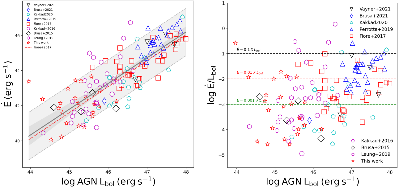
Fig. 12: Ionised kinetic power and kinetic coupling efficiency as a function of AGN bolometric luminosity. Left panel: Ionised kinetic power as a function of AGN bolometric luminosity. The red dashed line is the best scaling relation obtained in Fiore et al. (2017) . The solid grey line in both panels is our scaling relation obtained from OLS fitting between the two variables. The grey region indicates the 95% confidence interval and the faded filled region between two dashed black lines is the 1\sigma . Right panel: Kinetic coupling efficiency ( \dot{E}/L_{bol} ) versus AGN bolometric luminosity. The black dashed line represents \dot{E} = 0.1 L_{bol} , red dashed line represents \dot{E} = 0.01 L_{bol} and green dashed line represents \dot{E} = 0.001 L_{bol} . 30% of the candidates appear above \dot{E}/L_{bol}=0.01 or 1%. These values have 2-3 orders of magnitude uncertainties due to the different assumptions applied.
