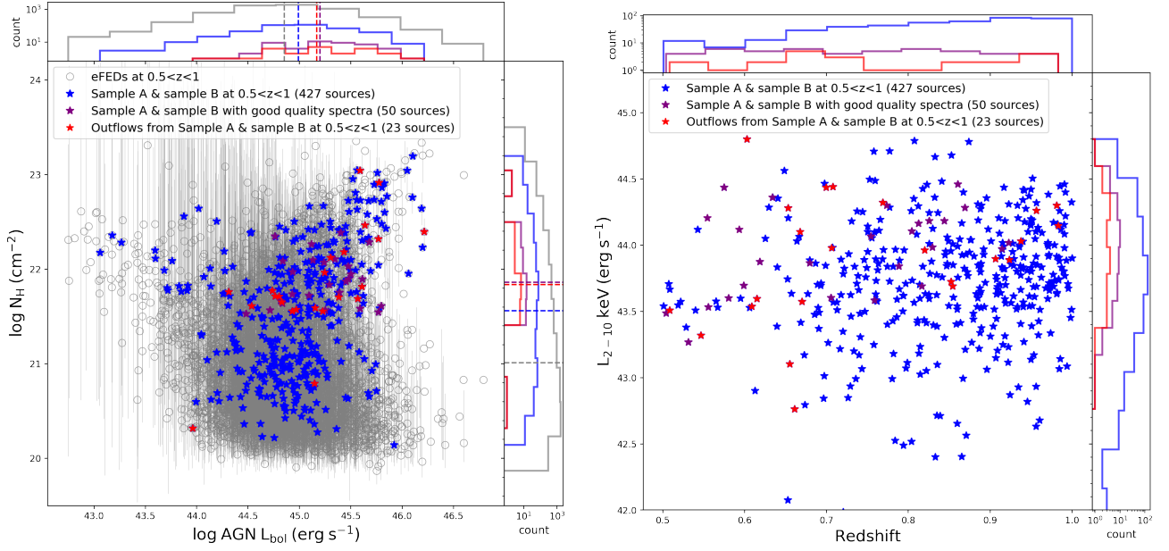
Fig. 9: Comparisons of the different samples. Left panel: N_H and AGN bolometric representation of our isolated candidates. Open grey circles represent eFEDS sources at 0.5 < z < 1 , blue-filled stars represent sample A and sample B at 0.5 < z < 1 , purple-filled stars represent sample A and sample B with good quality SDSS spectra and the red-filled stars represent the 23 candidates confirmed with outflows. The colours used in the histograms are identical to the colours used in the legend of the scatter plot for the same samples. The dotted lines represent the means of the respective distributions. Right panel: The X-ray luminosity and redshift distributions of three samples; sample A and sample B at 0.5 < z < 1 , sample A and sample B with good quality SDSS spectra and 23 candidates confirmed with outflows. The colours used in the histograms are identical to the colours used in the legend of the scatter plot for the same samples.
