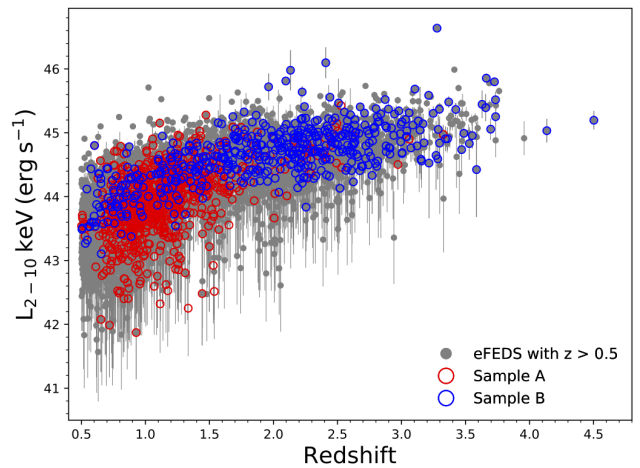
Fig. 5: X-ray luminosity and redshift distributions of our two main candidate samples. The grey points indicate the eFEDS AGN sample at z>0.5 . The red circles indicate sample A obtained after applying the colour selections described in Sect. 2.2 while blue circles indicate Sample B selected as detailed in 2.3.
