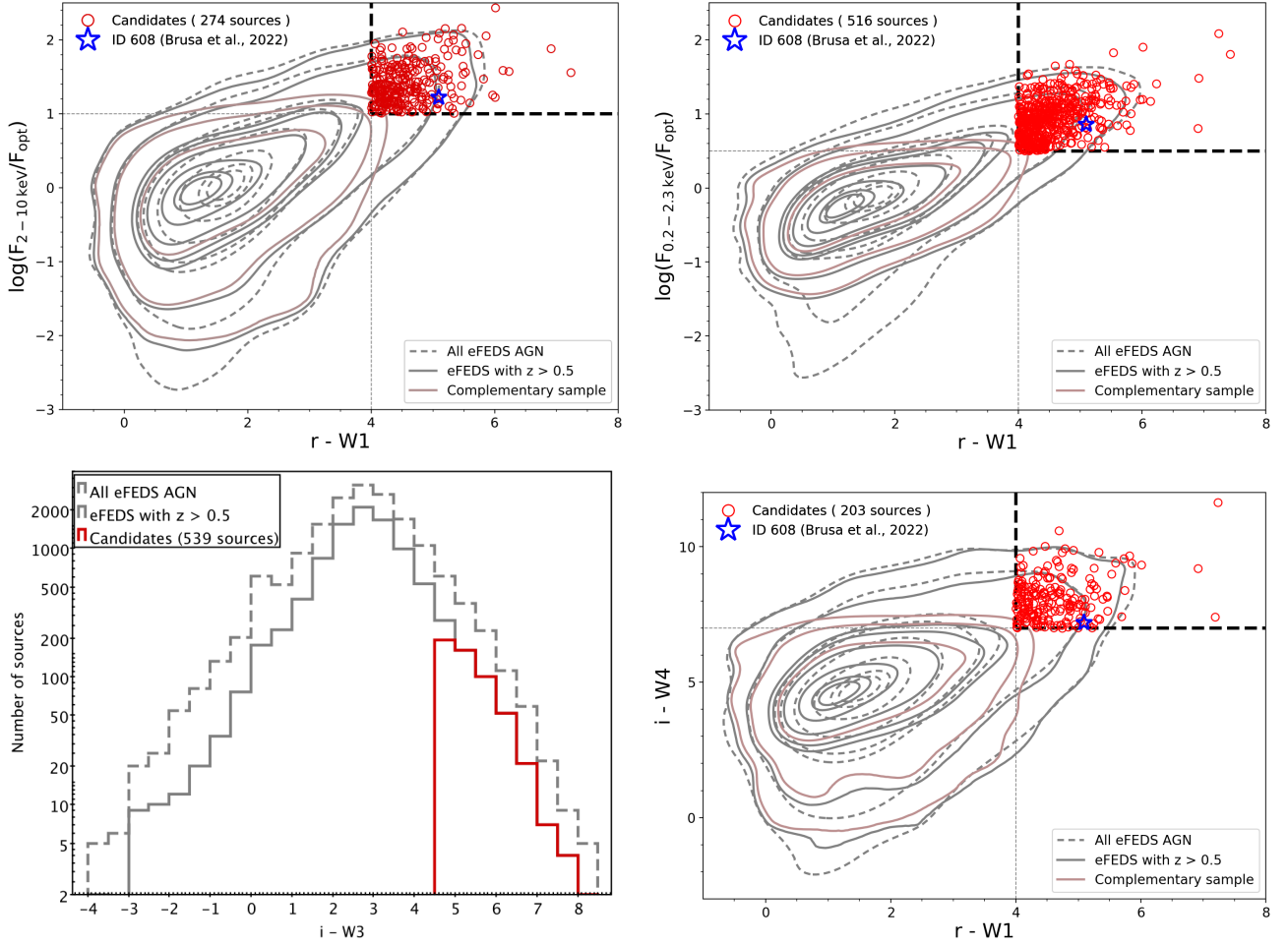
Fig. 1: Plots showing the colour selections to isolate AGNs in the feedback phase. Top left panel: The 2 – 10 keV to optical flux ratio versus r-W1 colour. The black thick dashed lines represent Eq. 3 and 1 selection locus. Top right panel: The 0.2 – 2.3 keV to optical flux ratio versus r-W1 colour. The black thick dashed lines represent Eq. 4 and 1 selection locus. Bottom left panel: Distribution of i-W3 selected sample. Red distribution are selected candidates with Eq. 2. Bottom right panel: i-W4 versus r-W1 selection method. The black thick dashed lines represent the Equations 5 and 1 selection locus. In all panels, the red circles are the selected candidates. Brown contours are sources in the complementary locus. Solid grey contours or distribution indicate the eFEDS AGN sample after applying the cut on redshift ( z > 0.5 ) and dashed grey contours or distribution show the full eFEDS AGN sample. XID 439 or ID 608 Brusa et al. (2022) is shown as a blue star.
