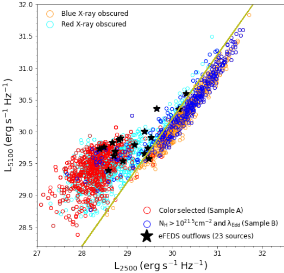
Fig. 7: Luminosity at 5100 Å ( L_{5100\text{\AA}} ) versus Luminosity at 2500 Å ( L_{2500\text{\AA}} ) for sources in Sample A and B. Representation of the selected samples with the X-ray obscured sources ( N_H > 10^{21.5}\text{cm}^{-2} ; red obscured and blue obscured based on the line L_{5100\text{\AA}} - L_{2500\text{\AA}} = 0.2 ; see Text for details). Candidates in sample B appear in the blue side (selects mostly type 1 AGN). It also correlates well with L_{5100\text{\AA}} - L_{2500\text{\AA}} = 0.2 relation which indicates their type 1 nature. Sample A indeed appear in the red side (selects mostly type 2 AGN). We indicate in black stars the 23 ionised outflows from the eFEDS sample (see Sect. 3.2 for the discussion of these 23 sources )
