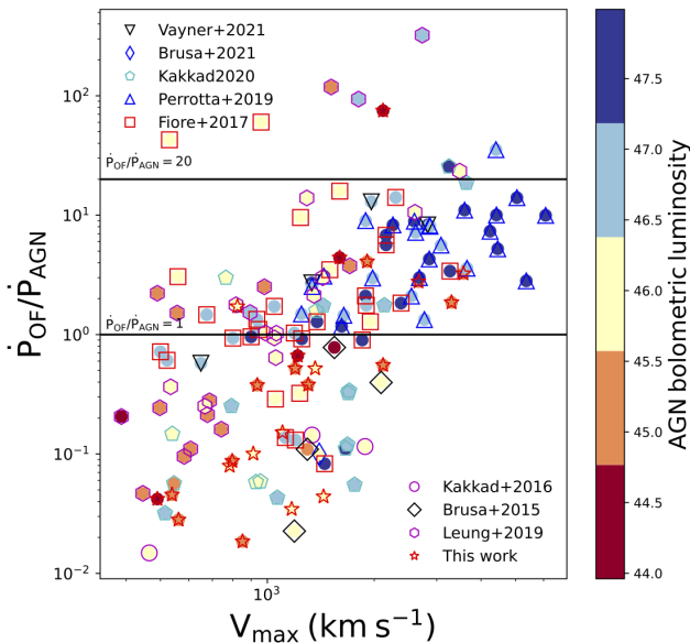
Fig. 13: We plot the outflow momentum rate (momentum flux of the outflow divided by the radiation momentum flux from the central black hole) against the maximum outflow velocity and colour-coded with the AGN bolometric luminosity. The black solid lines show the P_{\text{OF}}/P_{\text{AGN}} = 20 and =1 as indicated in the plot. The majority of our sources have momentum flux ratios of less than 20.
