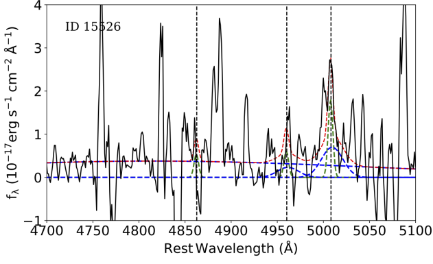
Fig. B.3: An example of the spectra that we classified as bad due to a very noisy continuum around the [OIII] region or bad residuals after the continuum and host galaxy subtraction. The red line indicates the total fit. The vertical dotted lines indicate the peaks at 4862.68, 4960.30, and 5008.24 for H_\beta and [OIII] rest-frame wavelength.
