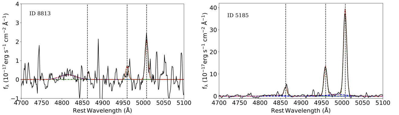
Fig. B.2: Examples of spectra from two component fit but with poor spectra and single component fit. Left panel: An example of the spectra with single component fit (ID 8813) and \text{FWHM} < 800 \text{ km s}^{-1} . Right panel: An example of the spectra with two component fit (ID 5185) but whose flux-to-flux error ratio is less than 2.5. These sources were excluded from our final candidates with outflows because the additional broad component is not significant. In both panels, the red line indicates the total fit. The vertical dotted lines indicate the peaks at 4862.68, 4960.30, and 5008.24 for H\beta and [\text{OIII}] rest-frame wavelength.
