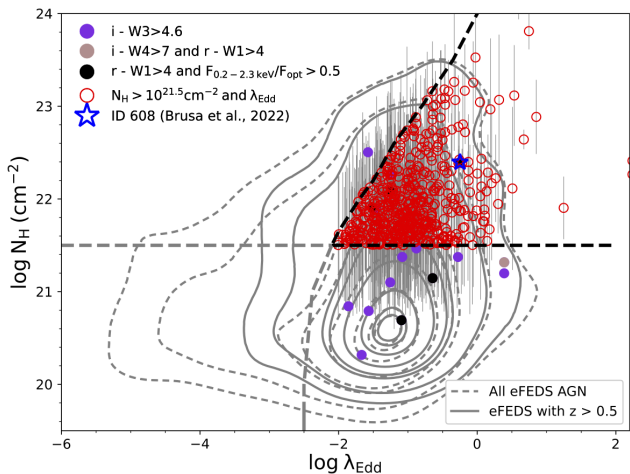
Fig. 2: N_{\text{H}} plotted against Eddington ratio. Sources marked in red are the selected candidates. Solid grey contours are eFEDS sample after applying the cut on redshift ( z > 0.5 ) and dashed grey contours show the full eFEDS sample. ID 608 (Brusa et al. 2022) (blue star) and the sources isolated from Sect. 2.2 are shown with violet circles. The black thick dashed line and curve represent the region N_{\text{H}} > 10^{21.5} \text{ cm}^{-2} and \lambda_{\text{Edd}} > \text{effective Eddington limit} . The dotted curve (thick and thin) is the effective Eddington limit for different values of N_{\text{H}} (Fabian et al. 2009).
