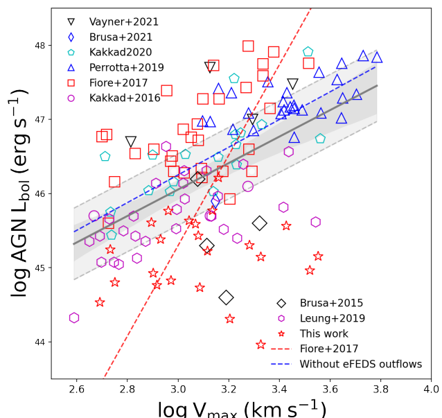
Fig. 10: AGN bolometric luminosity as a function of outflow velocity. Different shapes represent different samples from literature, as labelled. The solid grey line is the scaling relation obtained from fitting between the two variables including our AGN outflows from eFEDS (see Table 2). The grey region indicates the 95% confidence interval and the shaded filled region between two dashed black lines is the 1\sigma . The red dashed line is the scaling relation from Fiore et al. (2017), obtained for a sample of \sim 55 ionised outflows without imposing a redshift cut z > 0.5 . The blue dashed line is the scaling relation obtained from fitting the two variables excluding our eFEDS sources. The relation still appears flattish as compared to Fiore et al. (2017). It is important to note that we maintain the same legend for QWO and eFEDS sources in the following figures.
