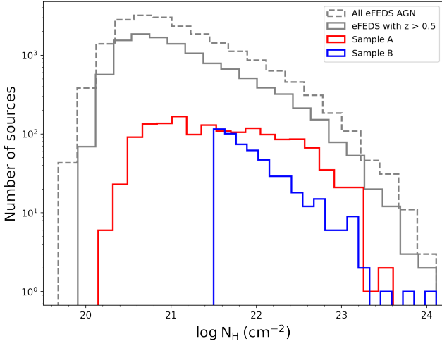
Fig. 6: N_H distribution of our selected candidates from the different methods compared with the overall eFEDS AGN sample and subsample at z > 0.5 . Our isolated candidates appear more obscured than the overall eFEDS AGN population and subsample at z > 0.5 .
