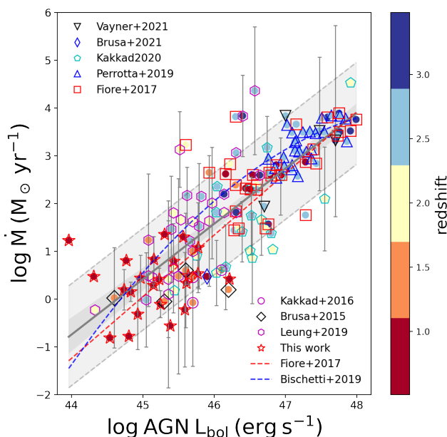
Fig. 11: Ionised mass outflow rate as a function of AGN bolometric luminosity. Different shapes represent different literature samples (as labelled). The filled circles are colour-coded with redshift. The blue dashed line is the best-fit relation obtained for ionised outflows in Bischetti et al. (2019). The solid grey line is the scaling relation obtained in this work, from fitting between the two variables (see Table 2). The grey region indicates the 95% confidence interval and the shaded filled region between two dashed black lines is the 1\sigma . The red dashed line is the scaling relation from Fiore et al. (2017), obtained for a sample of \sim 55 ionised outflows without imposing a redshift cut z > 0.5 . The error bars on mass outflow rate values were obtained by extrapolating the errors on FWHM or \delta V whenever available. These values may have 2-3 orders of magnitude uncertainties due to the different assumptions applied.
