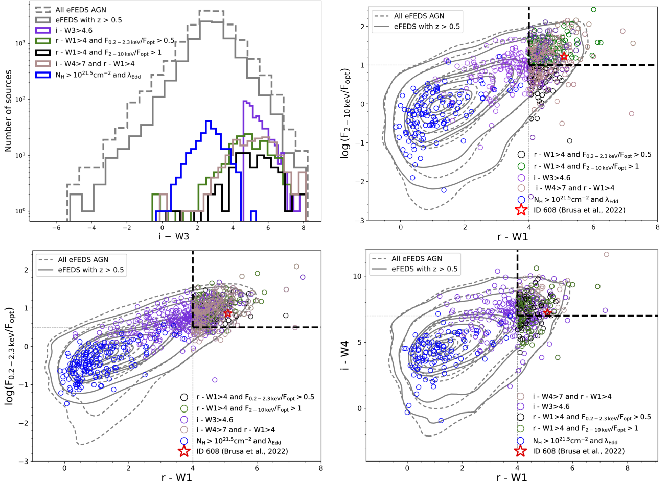
Fig. A.1: All selected candidates plotted in different planes. Top left panel: i - W3 distribution of candidates selected by different methods. Top right panel: Candidates selected by different methods plotted in 2 - 10 keV to optical flux ratio vs. r - W1 colour plane. Bottom left panel: 0.2 - 2.3 keV to optical flux ratio vs. r - W1 colour. The sources from different selection methods are indicated with different colours or shapes as shown in the legend. Bottom right panel: All selected candidates plotted in i - W4 vs. r - W1 . The sources from different selection methods are indicated with different colours as shown in the legend.
