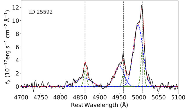
Fig. 8: SDSS emission line profiles fit of the H\beta + [OIII] line continuum subtracted complex for one of our candidates. The blue dashed line indicated the broad component, the green fit indicates the narrow component. The red dashed line indicates the total fit. The vertical dotted lines indicate the peaks at 4862.68, 4960.30, and 5008.24 for H\beta and [OIII] rest-frame wavelength.
