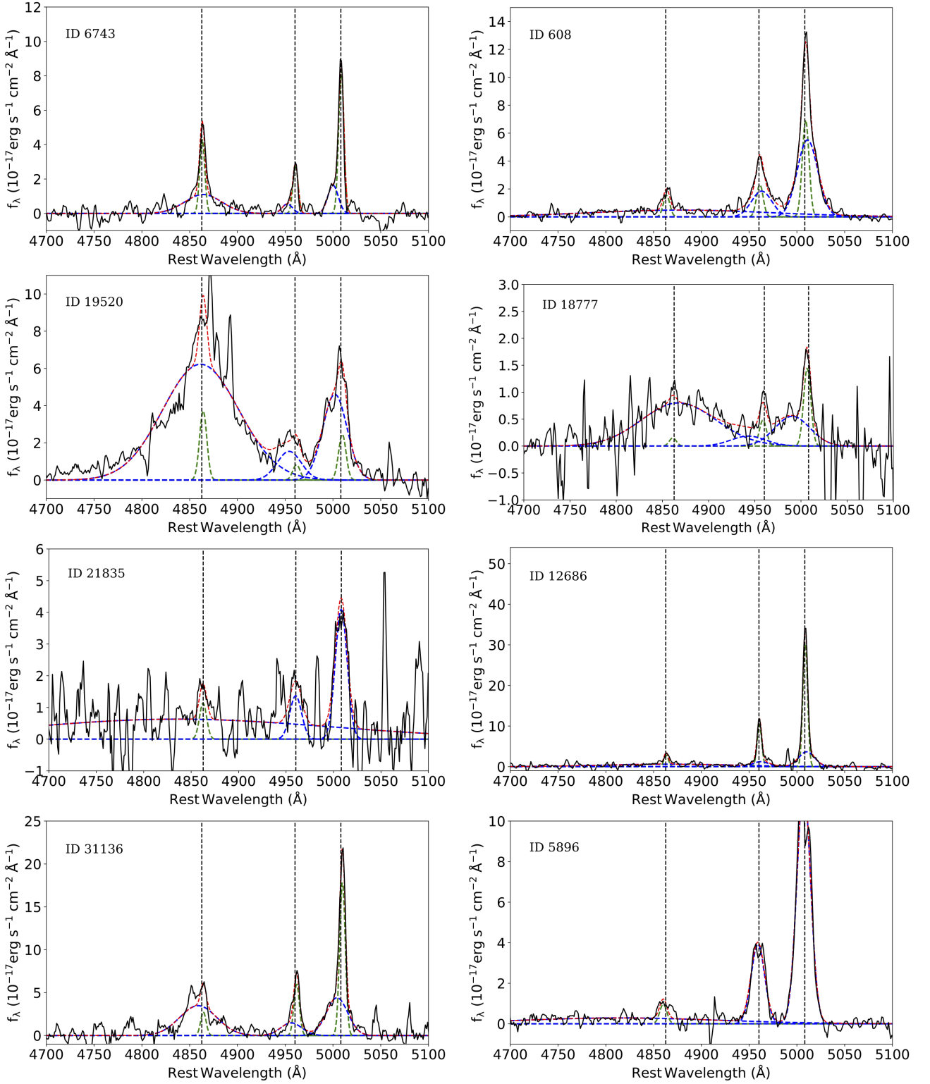
Fig. B.1: SDSS emission line profiles fit for our candidates with outflows. The blue line indicates the broad component and the green fit indicates the narrow component. The red line indicates the total fit. The vertical dotted lines indicate the peaks at 4862.68, 4960.30, and 5008.24 for H_\beta and [OIII] rest-frame wavelength.
