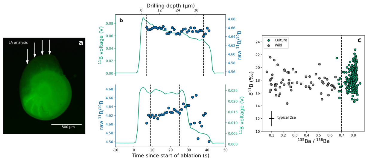
Fig. 1. Example boron and barium isotope analysis of cultured Operculina ammonoides using LA-MC-ICPMS. (a) Fluorescent microscope picture of a cultured O. ammonoides illustrating the use of calcein to identify chambers precipitated in the laboratory. The low fluorescence chambers (top) are those grown during the culture experiment. The direction of the laser ablation analyses is depicted by arrows. (b) Two examples of a time resolved laser ablation analysis. The dashed vertical black lines depict the locations at which the data was trimmed in the case of these specific samples. Both analyses were performed on cultured foraminifera using a laser spot size of 40 \mu\text{m} , a repetition rate of 6 Hz and a fluence of 6 \text{J}/\text{cm}^2 . The analysis on top is an example of a stable signal with no chamber breakage whilst the bottom shows a chamber breakthrough after around 29 s of laser drilling. Drilling depth was estimated using an ablation rate of 200 nm/pulse at 6 Hz, 6 \text{J}/\text{cm}^2 (Griffiths et al., 2013). (c) Example use of ^{135}\text{Ba}/^{138}\text{Ba} to unambiguously identify material grown in laboratory culture, plotted against \delta^{11}\text{B} at an adjacent locations in the shell (the Ba isotope analyses were laterally offset by \sim 20\ \mu\text{m} from the boron isotope analyses, see text for details). The vertical dashed line delineates the cut-off point representing a value 10 % lower than the culture ^{135}\text{Ba}/^{138}\text{Ba} endmember. The green data points are those that are within uncertainty of the cut-off point, considered to have come from material grown under the experimental conditions.
