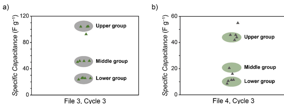
Fig. 6. Specific capacitance results ( F g^{-1} ) collected from participating groups for (a) File 3 (ideal), where three distinctive groups of reported values are seen, and (b) File 4 (non-ideal), where three groups of values are also present. The mean value for the upper group in File 3 is 104.9 F g^{-1} . The mean value for the lower group in File 3 is 26.0 F g^{-1} . The mean value for the upper group in File 4 is 44.7 F g^{-1} . The adjusted mean value for the lower group in File 4 is 10.8 F g^{-1} . The mean value for the middle group is not reported as these values have been calculated using incorrect equations.
