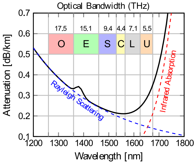
Figure 11. Typical fiber attenuation spectrum for a low-water peak single-mode silica fiber and corresponding transmission bands from O- to U-band.
