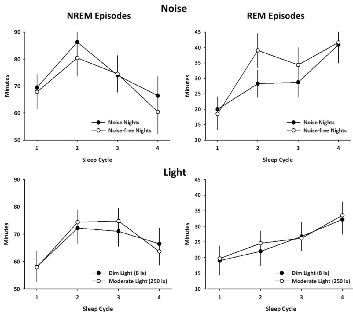
Fig. 4. Influence of noise (upper panel) and light (lower panel) on the duration of NREM and REM sleep episodes in minutes over four sleep cycles. Values represent estimated means \pm 95% confidence intervals based on generalized linear mixed model (GLMM). The GLMM yielded no significant effects of the modulators “noise” and “light” or their interaction with “sleep cycle” (see Table 1 for details).
