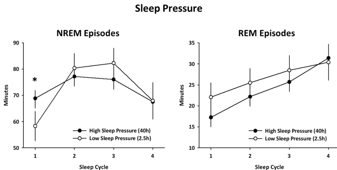
Fig. 5. Influence of high and low sleep pressure on the duration of nonrapid eye movement (NREM) and rapid eye movement (REM) sleep episodes in minutes over four sleep cycles. Values represent estimated means \pm 95% confidence intervals based on generalized linear mixed model (GLMM). The low sleep pressure condition was achieved with a nap protocol, while the high sleep pressure condition was achieved with 40 hours of sleep deprivation. A significant main effect “sleep pressure” was found for the duration of REM sleep episodes, with higher values in low than in high sleep pressure conditions. For NREM sleep episode duration, a significant “sleep pressure” \times “sleep cycle” effect was found (see Table 1 for details), with a longer duration under high than low sleep pressure conditions in the first sleep cycle. The asterisk indicate significant post-hoc comparisons after correction for multiple testing (Tukey-Kramer, p < .05 , only when GLMM indicated a significant modulator \times sleep cycle effect).
