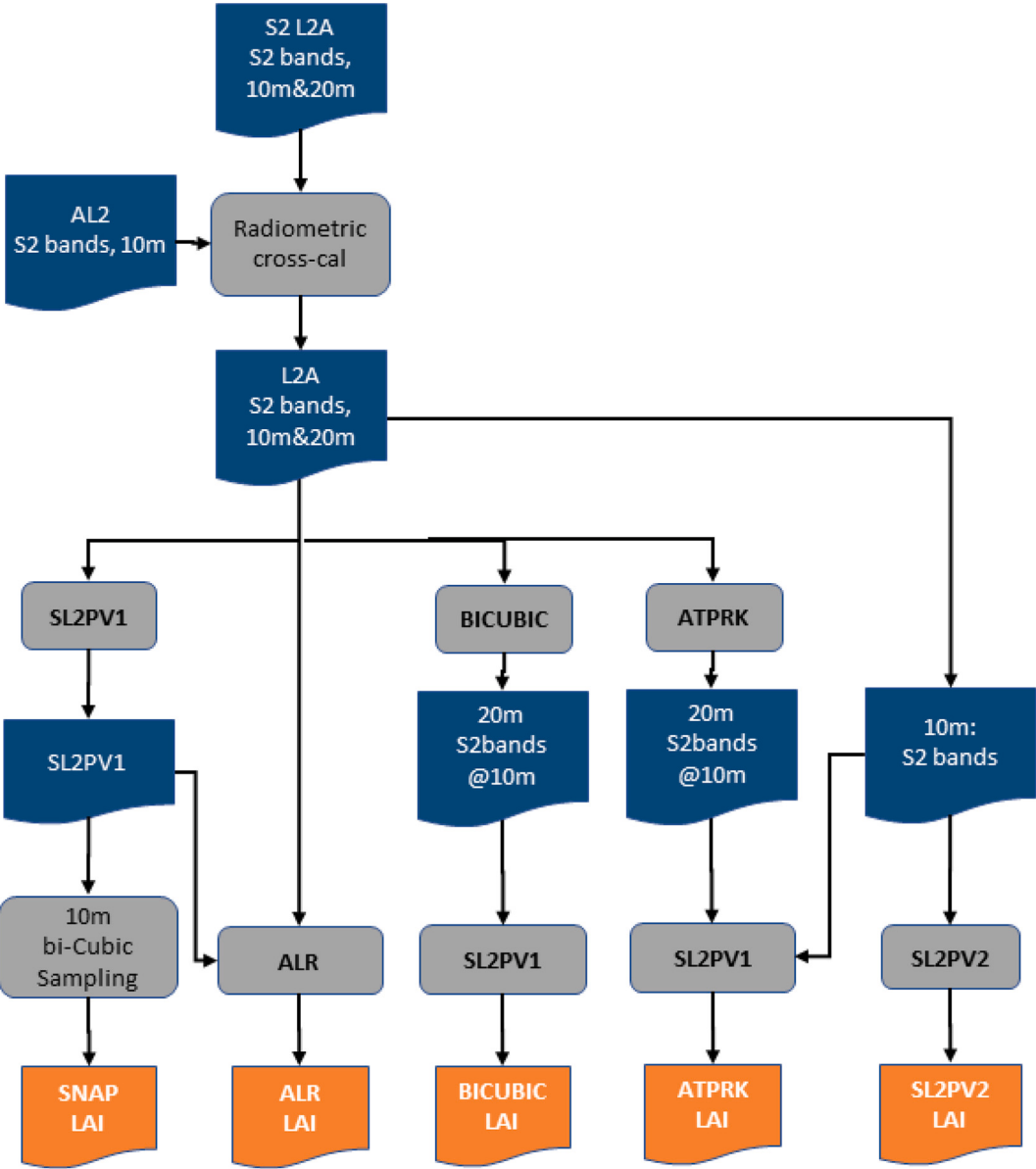
Appendix B. Flowchart of methods for deriving downscaled products from L2 imagery
