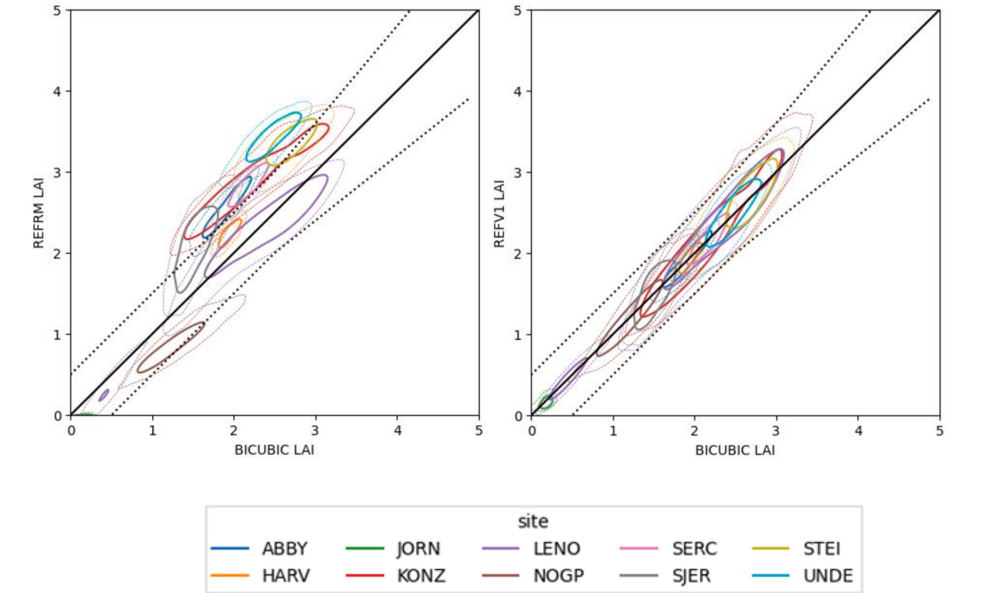
Fig. F1. Kernel density plots of estimated 10 m LAI from 20 m resolution AL2 imagery versus REFRM 10 m LAI (left panel;) and REFV1 10 m LAI (right panel) for each site. Solid (dashed) contours correspond to 50 percentile (10 percentile) cumulative probability density. Dashed line corresponds to GCOS LAI uncertainty requirement, solid line corresponds to 1:1 line.
