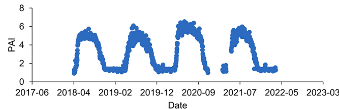
Fig. A1. Time series of PAI derived from an automated DHP system installed at Wytham Woods, demonstrating little change in leaf-off PAI (i.e. WAI) between 2018 and 2022. Further details on the automated DHP system and data processing are provided by Brown et al. (2020b). (For interpretation of the references to colour in this figure legend, the reader is referred to the web version of this article.)
