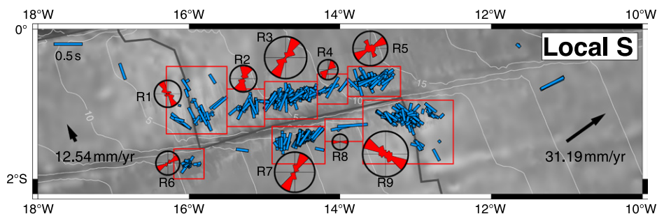
Figure 3. Map of local event shear wave splitting results (blue bars) plotted at the event-station midpoints. Rose diagrams indicate polarization direction of the fast shear wave ( \phi ) weighted by delay time ( \delta t ) for the bins (red boxes). Absolute plate motions are shown with black arrows.
