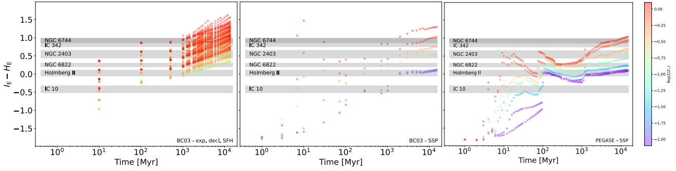
Fig. 7. Synthetic I_E - H_E from the Bruzual & Charlot (2003) models with exponentially declining SFH (left panel); the same Bruzual & Charlot (2003) models but SSPs (middle); and PEGASE SSP models from Fioc & Rocca-Volmerange (1997) , right) and Le Borgne et al. (2004) . The SSP models have no internal extinction applied to the colors. Also shown as gray regions are the mean I_E - H_E colors and their standard deviations, as reported in the middle panel of Figs. 6 and C.1, evaluated over a factor of 100 in galactocentric radius. As discussed in Sect. 4.1, these colors have been corrected for foreground extinction from our Galaxy. The different behavior of the models is due to the smoothed-out SFH in the left panel, and the different treatment of red supergiants that begin to dominate around 10 Myr, and the most massive AGB stars around 100 Myr.
