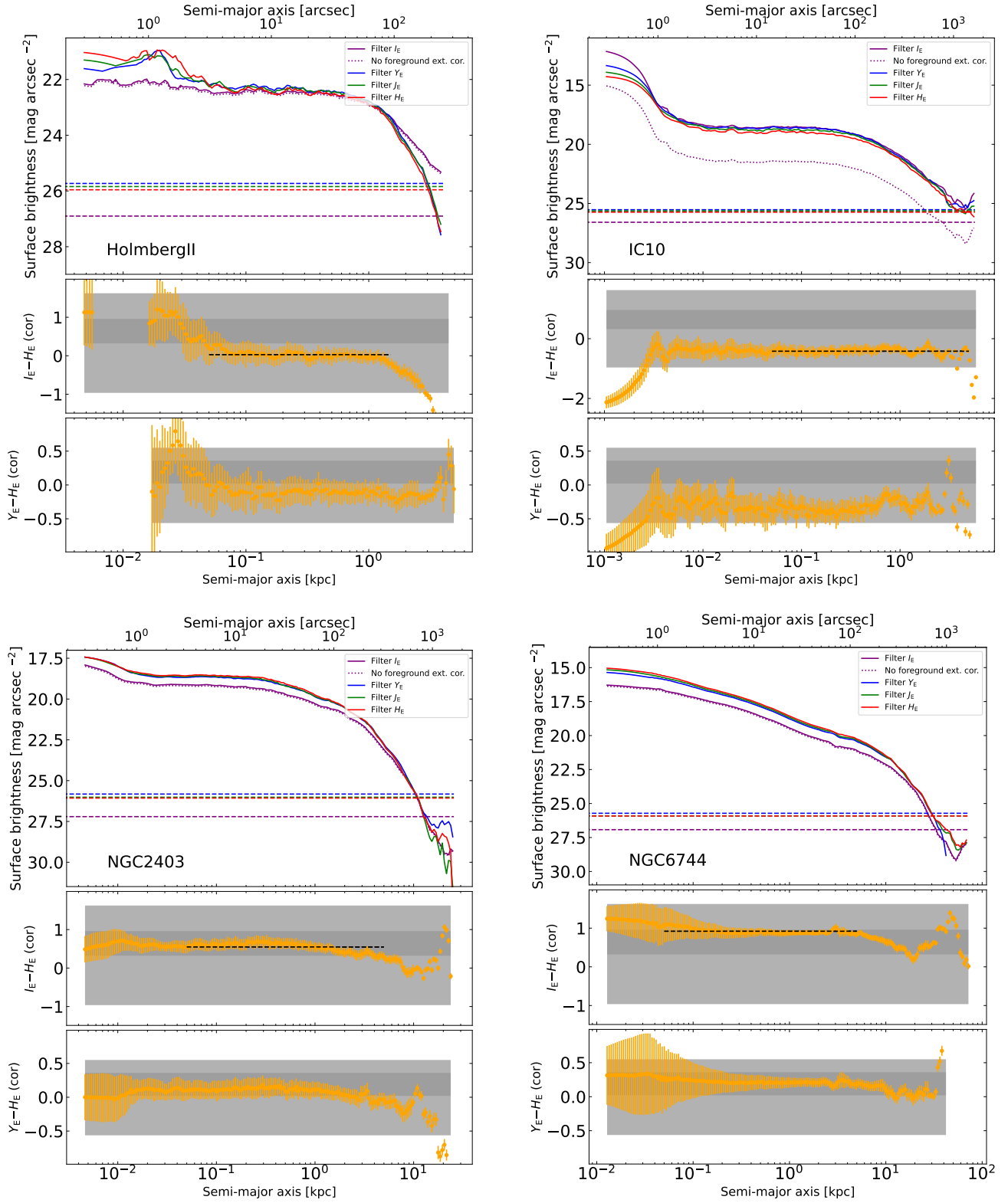
Fig. C.1. Surface brightness and color profiles extracted by AutoProf, as described in the text: Holmberg II and IC 10 in the top row; and NGC 2403 and NGC 6744 in the bottom. The four bands are given by purple, blue, green, and red for I_E , Y_E , J_E , and H_E , respectively. The 1 \sigma SB limits from AutoProf in units of mag arcsec -2 are shown as dashed horizontal lines, with colors corresponding to the Euclid bands. The fluxes have been corrected for foreground extinction (Sect. 4.1) in order to be consistent with the I_E - H_E radial color gradient shown in the middle panel, and Y_E - H_E shown at the bottom. The uncorrected I_E profile is shown as a dotted (purple) curve in the top panel. The mean I_E - H_E color over typically a factor of 100 in radius in the inner galaxy is shown as a horizontal dashed line in the middle panel.
