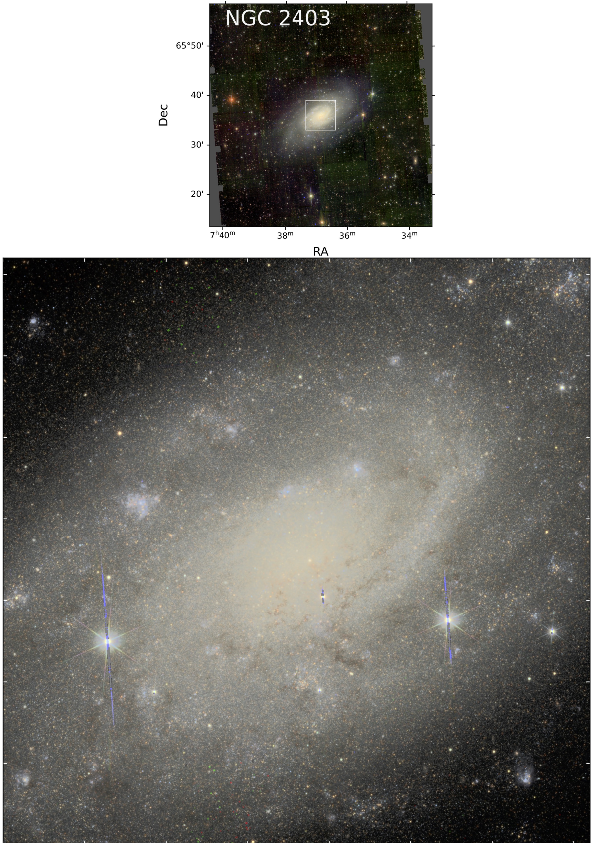
Fig. B.2. Same as for Fig. 1, but for NGC 2403.
