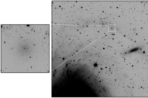
Fig. 16. Confirmation image of a previously identified dwarf satellite of NGC 6744, dw1909m6341; the image on the left is 50'' \times 50''. The larger 12' \times 12' image on the right shows its location near a dense stellar region that belongs to one of the spiral arms of the galaxy. The images are oriented with north up, and east to the left.
