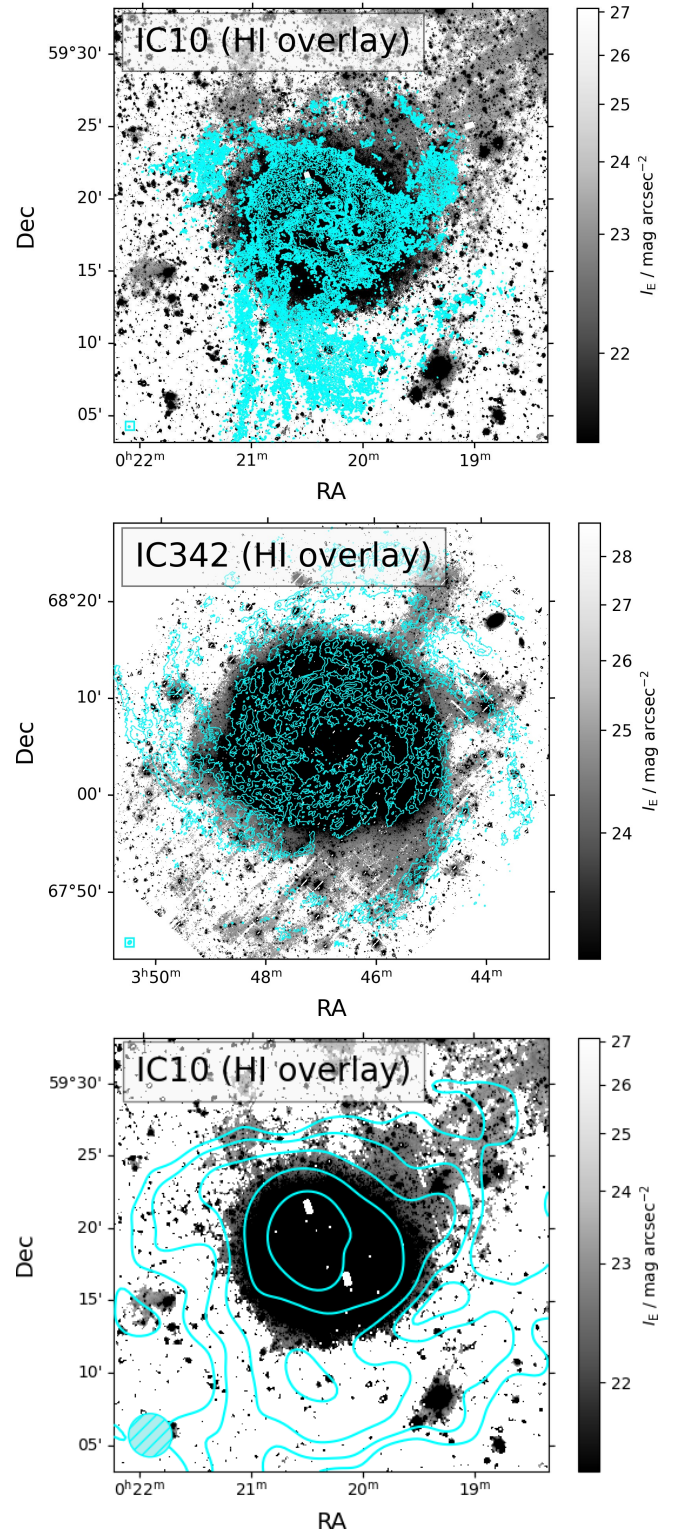
Fig. 4. H I overlays on high-contrast Euclid I_E images: IC 10 (top panel); and IC 342 (middle). The H I beam size is shown in the lower left corner, and contours are at 2\sigma , 4\sigma , 7\sigma , 10\sigma , and 20\sigma . The bottom panel gives the H I overlay for IC 10 as in the top panel, but using the 3-arcmin beam-smoothed H I image from Namumba et al. (2019) ; contours are at 2\sigma , 3\sigma , 5\sigma , 10\sigma , 10\sigma , and 70\sigma .
