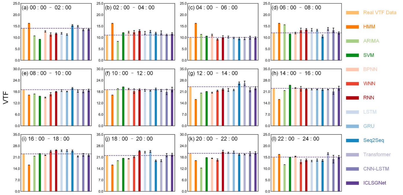
Fig. 24. The VTF prediction results (average value \pm standard deviation) for 12 different periods from time point 1093 (00:00–02:00) to 1104 (22:00–24:00) on September 30, 2020 in dataset C_7 .
