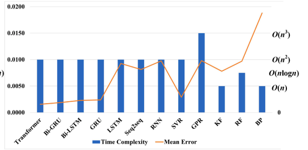
(b) the result of time complexity and mean error in the first dataset
