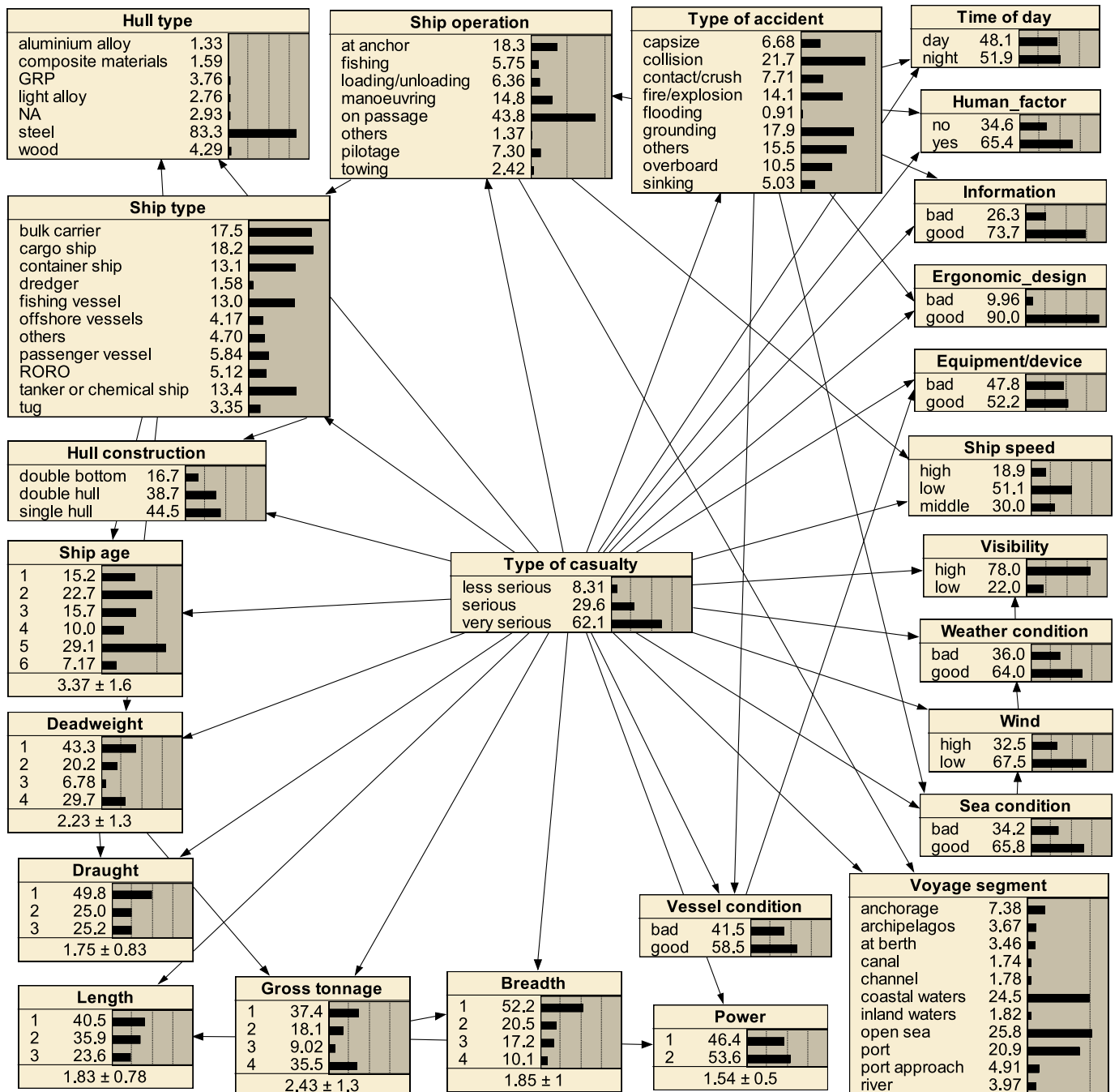
Fig. 14. A novel TAN with the ‘type of casualty’ as a parent node.
