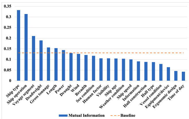
Fig. 6. Mutual information values of RIFs.
