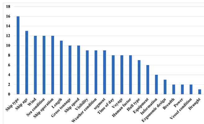
Fig. 1. The frequency of RIFs from the screened papers.
