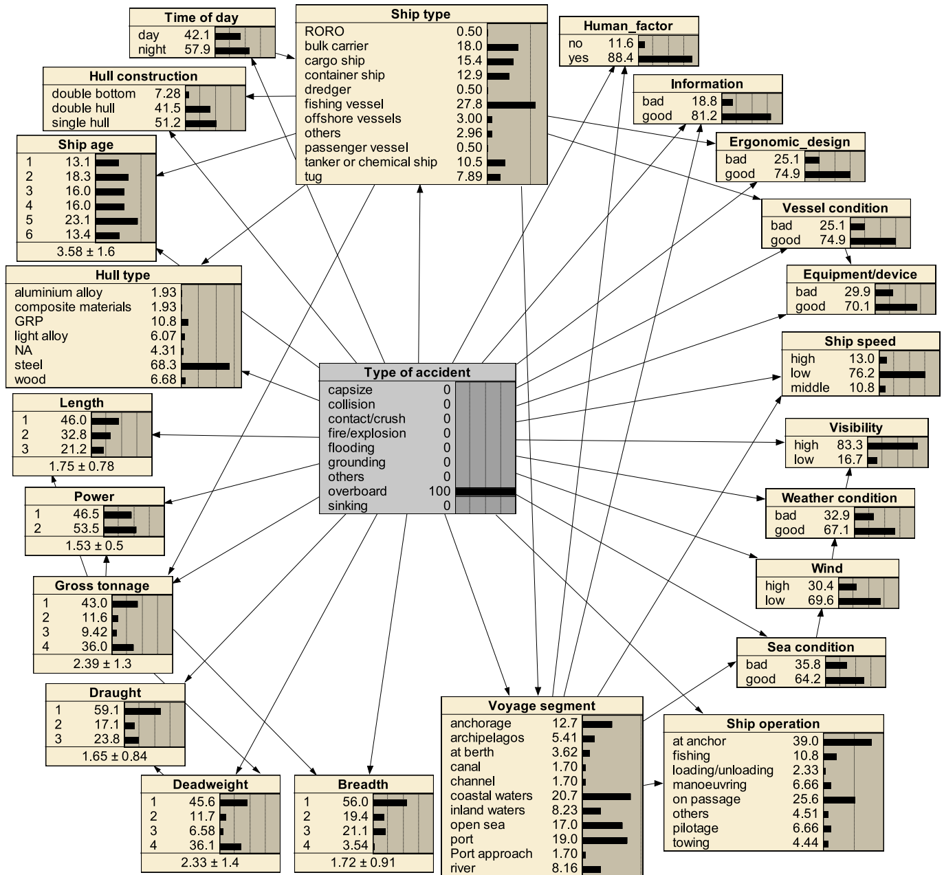
Fig. 11. The most probable scenario for overboard in this study.
