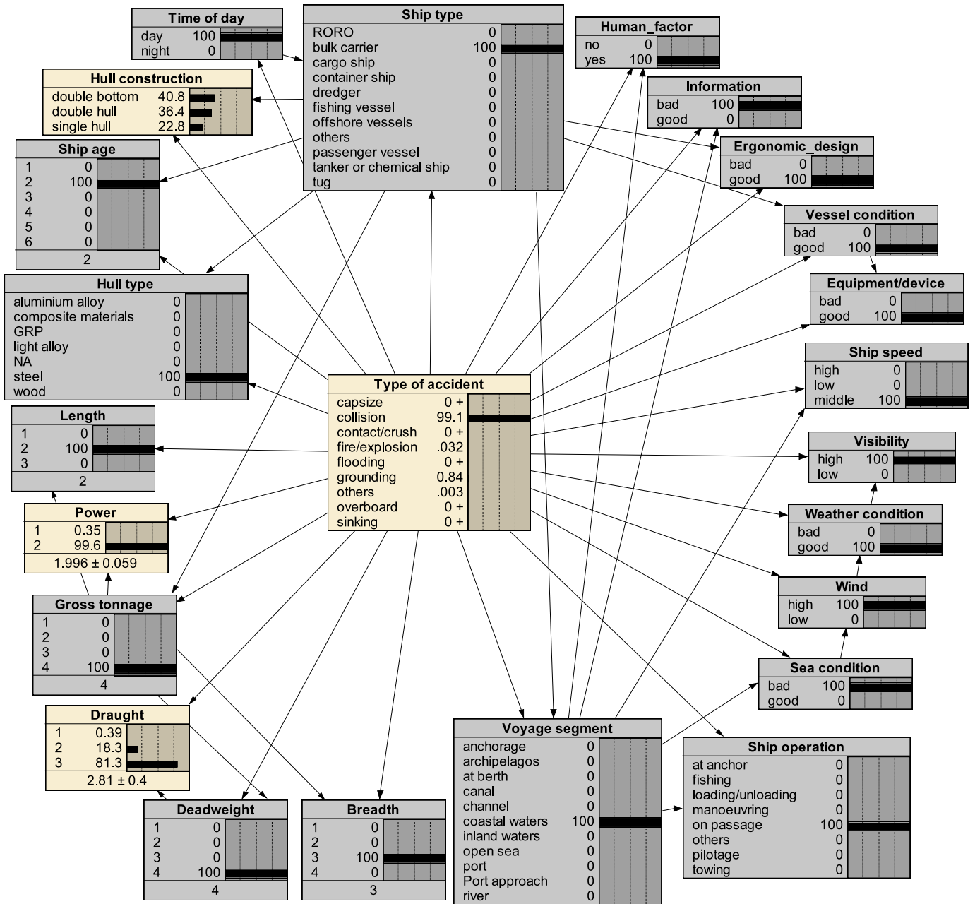
Fig. 8. A real case validation in 2022 by the constructed data-driven BN network.
