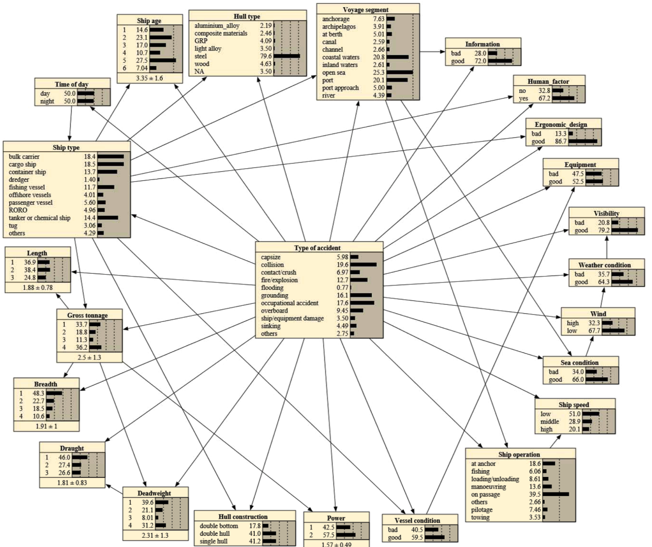
Fig. 4. The final TAN-based BN for the global maritime risk model.
