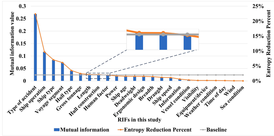
Fig. 5. Mutual information values and changes.
