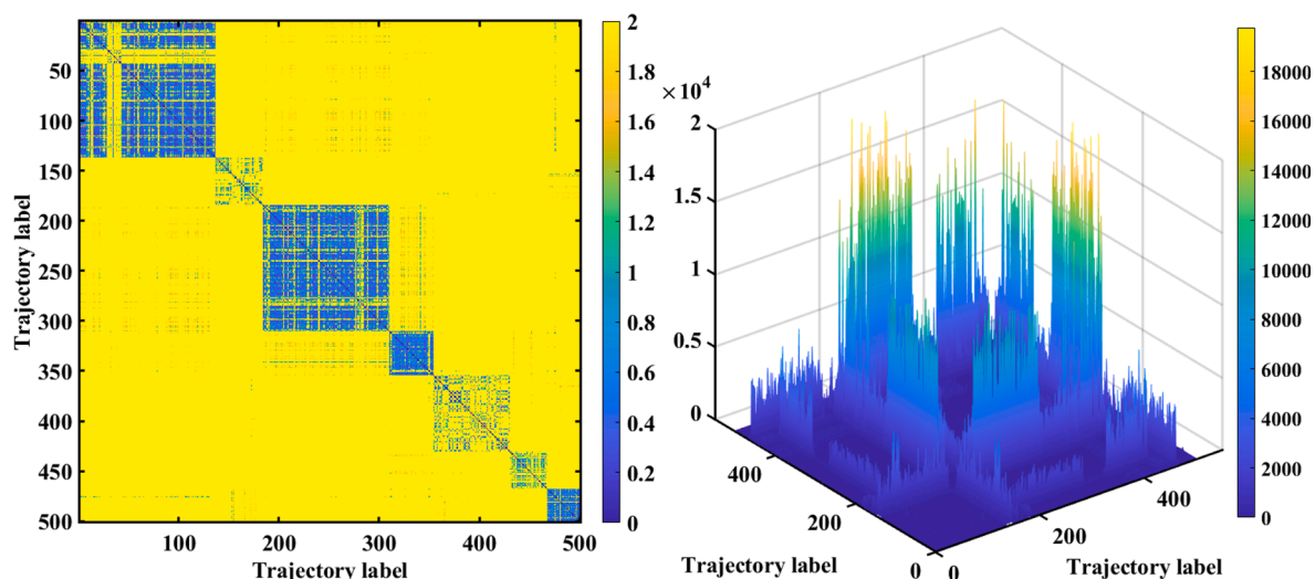
Fig. 17. Visualization of 2D and 3D results of the AADTW feature extraction method.
