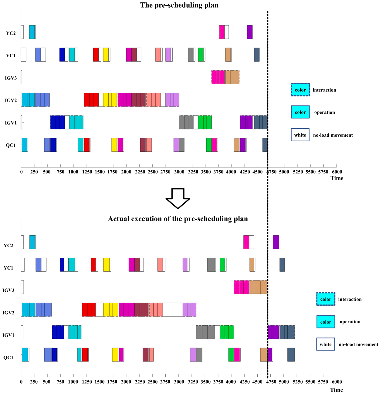
Fig. 3. Scheduling plans with operational time fluctuations.
