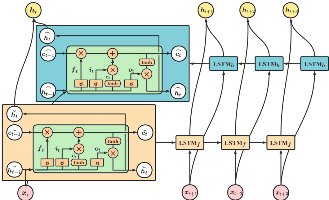
Fig. 2. The framework of the BiLSTM.
