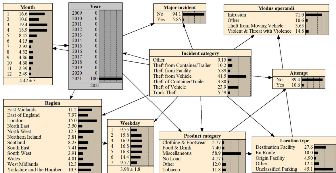
Fig. 7. Prediction results of TAN.
