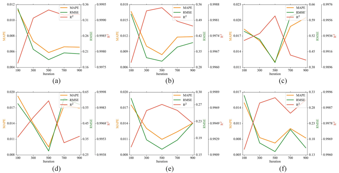
Fig. 10. The prediction results of the proposed MPTNSR model for three indices (i.e., RMSE, MAPE, and R^2 ) across five different iterations (i.e., 100, 300, 500, 700, and 900) in the CFPD water area. (a) – (f) indicate datasets C_1 – C_6 , respectively.
