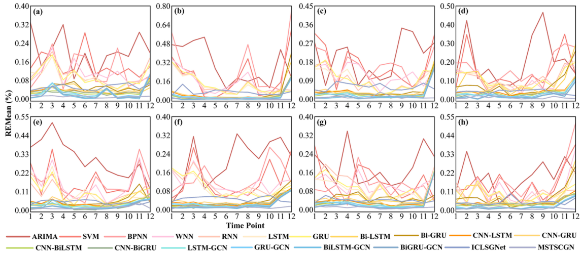
Fig. 15. The visualisation results of REMean using 19 different comparison methods in the CJ water area. (a) – (h) indicate datasets CJ 1 – CJ 8 , respectively.
