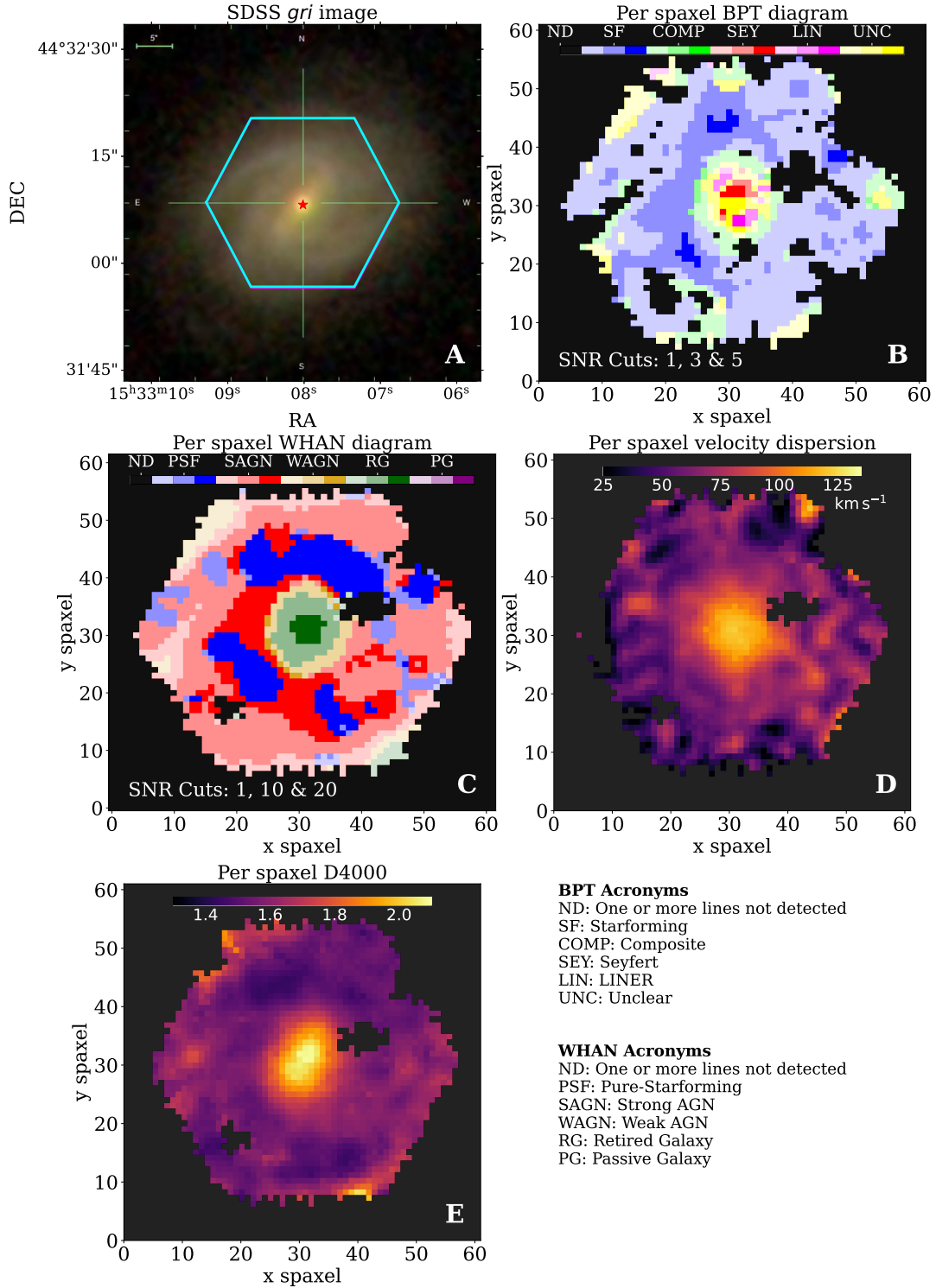
Figure 10. A: SDSS gri composite image of SDSS J1533+4432. Hexagonal outline displays the footprint of the MaNGA IFU data. B: Per spaxel combined BPT diagram of SDSS J1533+4432. Colour intensity indicates the SNR of the included emission lines in three bins at SNRs of 1, 3, and 5. Classifications use all four standard BPT diagnostic line ratios. BPT diagnostics cannot provide a clear classification for the emission line properties at the location of AT 2018dyk. C: Per spaxel WHAN diagram of SDSS J1533+4432. Colour intensity indicates the SNR of the included emission lines in three bins at SNRs of 1, 10, and 20. The WHAN diagram returns a clear (SNR of all lines >20) ‘retired galaxy’ (RG) classification for the nuclear region of SDSS J1533+4432, including the location of AT 2018dyk, indicating the LINER emission features are produced by an older stellar population rather than AGN activity. D: Per spaxel map of the measured stellar velocity dispersion (measured in \text{km s}^{-1} ) of SDSS J1533+4432. Overall velocity dispersion is within the range, though above the mean, of the velocity dispersions of TDE hosts found by Graul et al. (2018) . E: Per spaxel map of the measured D4000 spectral indices within SDSS J1533+4432. The increasing magnitude of this value moving radially towards the centre of the galaxy is consistent with increasing average stellar age. The spiral arms observable in both optical imaging and through BPT diagnostics are visible as the dark coloured regions above and below the galactic nucleus.
