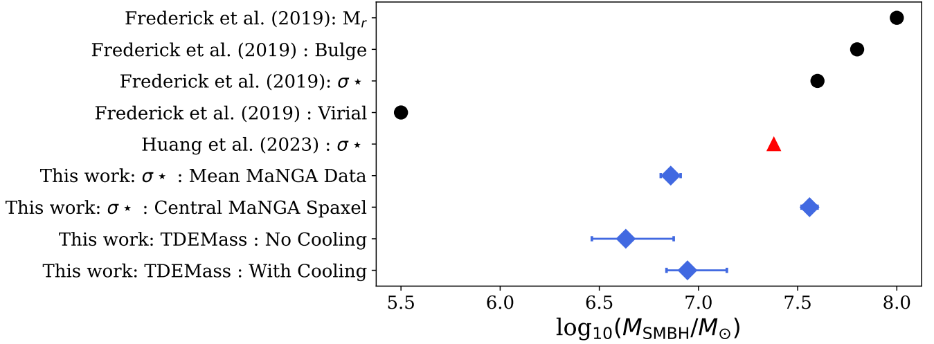
Figure 11. Compiled mass estimates for the SMBH at the centre of AT 2018dyk’s host galaxy. Data collated from Frederick et al. (2019) , Huang et al. (2023) , and this work. Note that the error bars reflect measurement uncertainties (where available) only and do not include any statistical uncertainties resulting from intrinsic scatter in the relations used.
