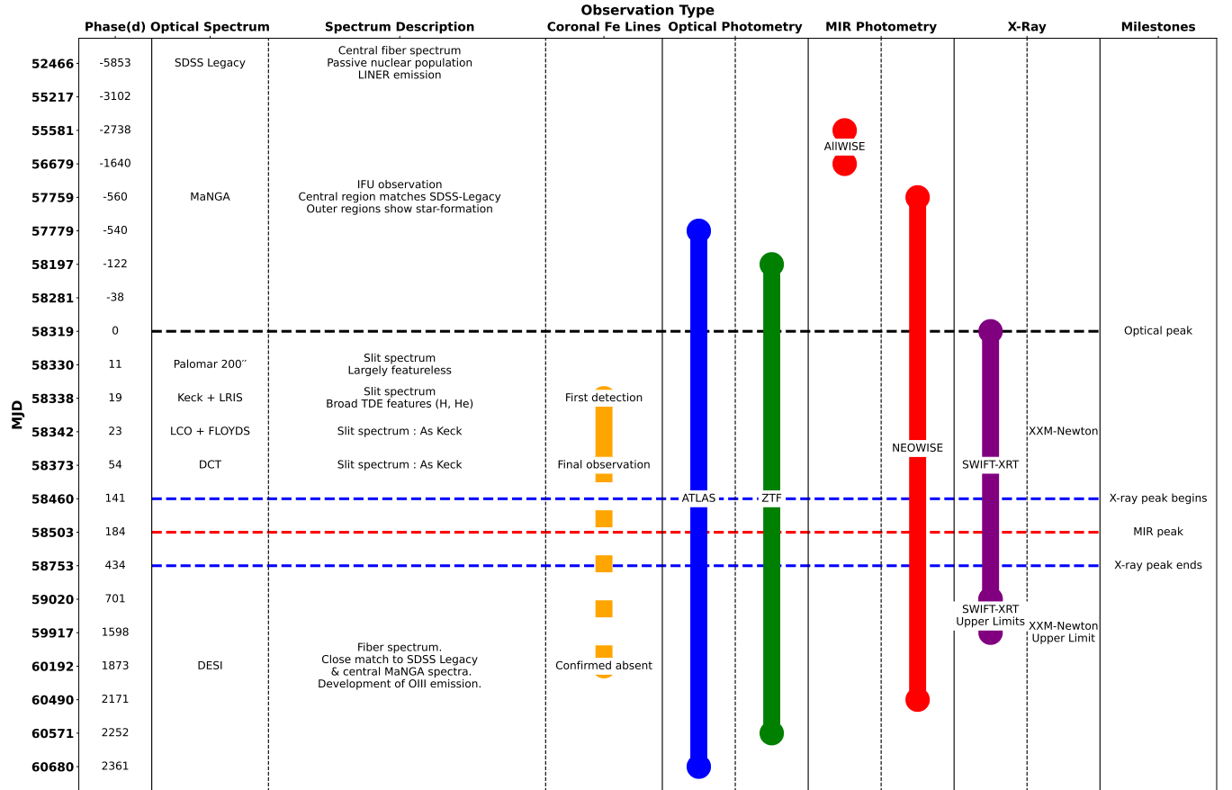
Figure 1. A visual summary of the available observations of AT 2018dyk. Additional optical spectra displaying typical TDE-like evolution and broad features exist between the LCOGT+FLOYDS spectrum and the DCT spectrum. All show similar coronal and other emission features. As these have not been made available publicly, we do not utilise them further in this work. Two observations of HST UV spectra were also obtained at phases of +182 and +226 d. We do not make use of these spectra within this work as there are no comparable observations for the other objects in the sample. The additional optical and UV spectra can be viewed in Frederick et al. (2019) .
