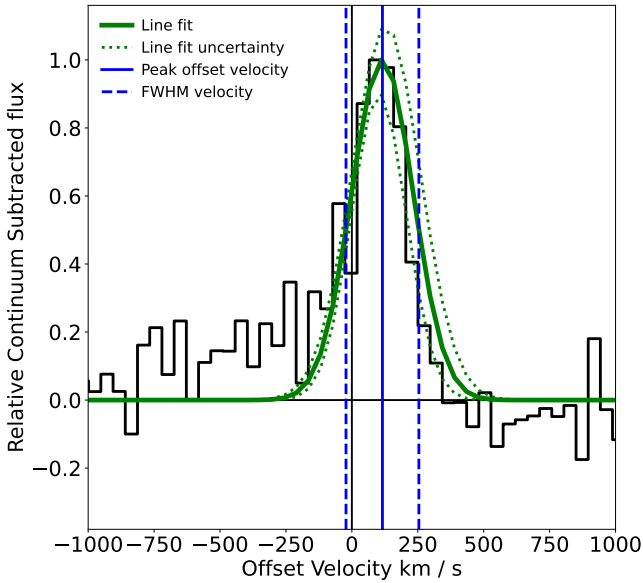
Figure 13. Fit to the [O III] 5007 Å emission line in the DESI spectrum of AT 2018dyk.
