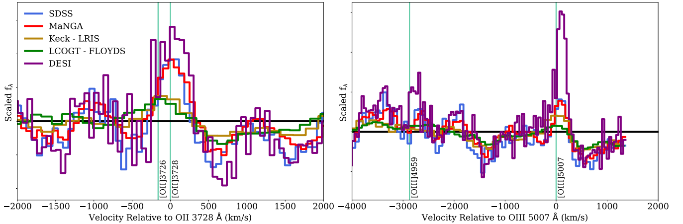
Figure 12. Left: [O II] 3726+3728 Å doublet line region in velocity space relative to the expected rest position of [O II] 3728 Å. The relative intensity of the feature drops during outburst before increasing in strength, exceeding the relative intensity of the feature prior to the original outburst. Right: Line region of the [O III] 4959 and 5007 Å lines in velocity space relative to the expected position of [O III] 5007 Å. The [O III] 4959 Å line is only observable in the most recent DESI spectrum. A sharp increase in [O III] 5007 Å emission is clearly observable in the most recent DESI spectrum. Slight redshifts ( \sim 100 \text{ km s}^{-1} ) in the observed line peaks are seen in both line regions. These are explored in detail in Section 4.1.
