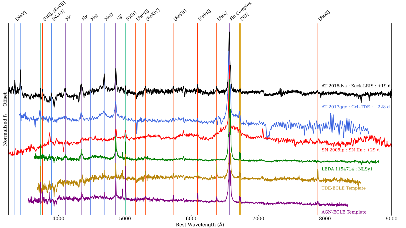
Figure 5. Comparison between the Keck+LRIS spectrum (obtained 19 d following optical peak) to a range of comparison objects. The AT 2018dyk spectrum shows similar coronal line features as those seen in the CrL-TDE AT 2017gge and in the ECLE templates (composite spectra obtained by combining the SDSS Legacy spectral observations of the sample) from Clark et al. (2024) , though at lower relative strength than the ECLE templates. The broad TDE features of H, He I, and He II are also shown by both AT 2018dyk and AT 2017gge. The spectrum of AT 2017gge is from a later phase relative to maximum light compared to AT 2018dyk as the coronal line features of AT 2017gge developed \sim 200 d post maximum light (as opposed to the near maximum light line emergence in AT 2018dyk). Such features are absent from the TDE-ECLE template as this is composed of spectra at much later relative phases (several years). The Type IIN SN 2005ip displays coronal emission at a much lower intensity than AT 2018dyk and the rest of the comparison sample. It also has a much broader H \alpha emission component but lacks the He I, He II, H \gamma , and H \delta emission lines.
