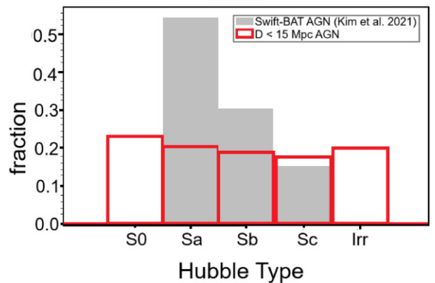
Figure 16. The distribution of Hubble type for our sample (red) and the Swift -BAT sample (grey; Kim et al. 2021).
