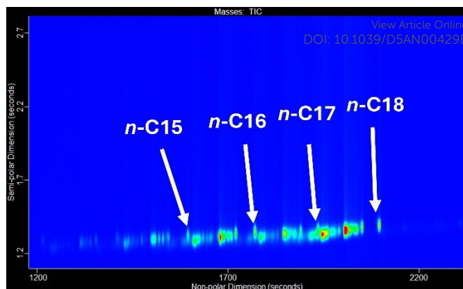
Figure 2: Two-dimensional total ion current chromatogram (TIC) contour plot of the GCxGC-MS analysis of diluted HVO 1.
