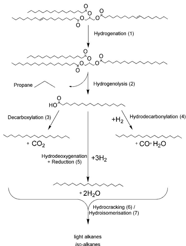
Figure 1: Simplified reaction scheme for the production of HVOs from triacylglycerides.
