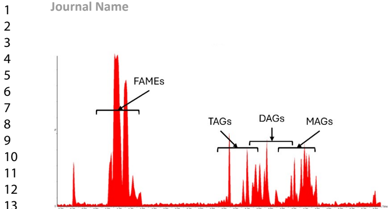
Figure 10: Base peak ion current chromatogram (BPIC) of the positive ion ESI SFC-MS for HVO 6.
