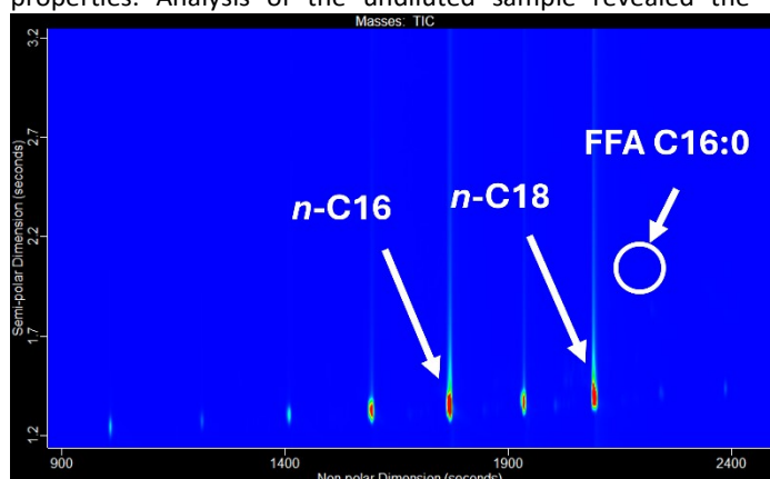
Figure 4: GCxGC-MS TIC contour plot of HVO 3-diluted (left). Note: overloading observed in the second dimension. 70 eV EI-MS and NIST 2017 library match of hexadecanoic acid (C16:0) detected in the sample (right).
