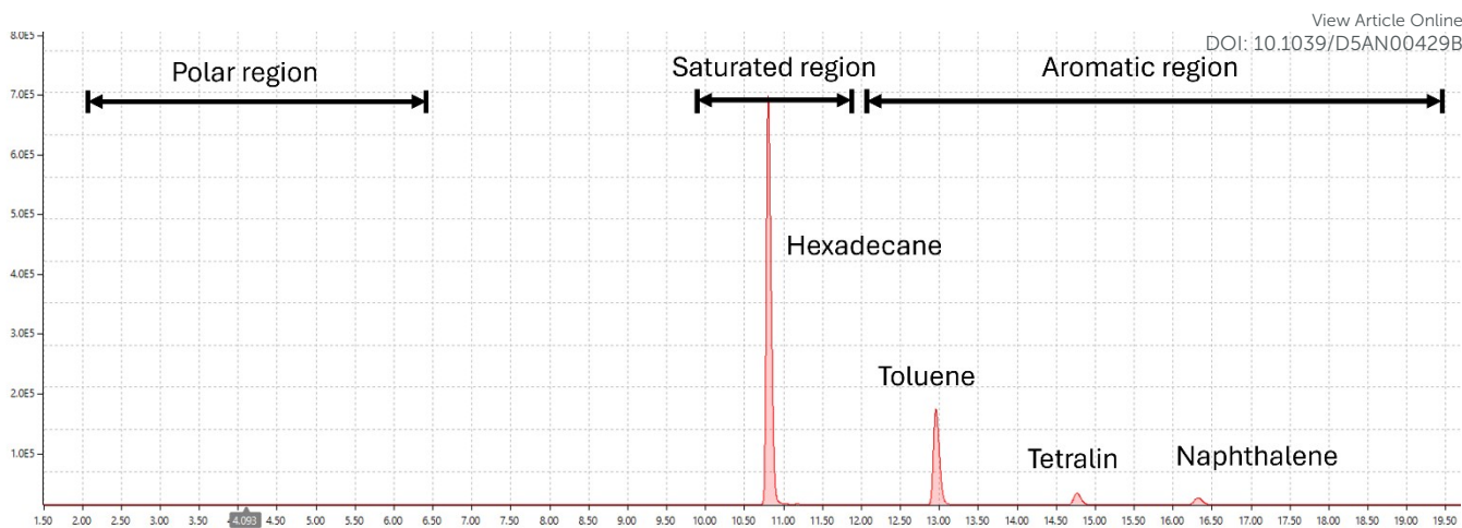
Figure 6: SFC-FID chromatogram of a standard mix showing group separation regions.
