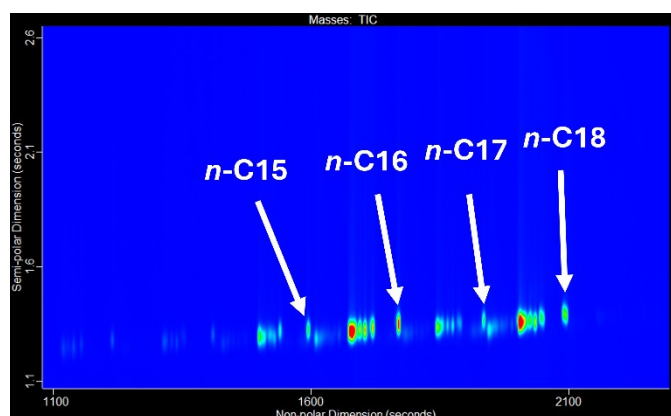
Figure 3: Two-dimensional TIC contour plot of the GCxGC-MS analysis of HVO 2-diluted.
