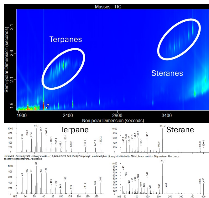
Figure 9: GCxGC-MS contour plot (top) and one example of the EI mass spectra and library match spectra of one terpene and one sterane detected in undiluted HVO 4 (bottom).
