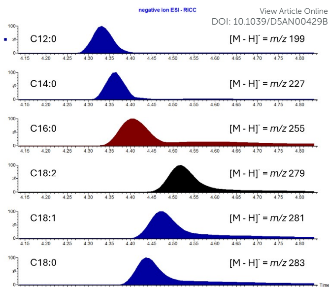
Figure 5: Reconstructed ion current chromatogram (RICC) of the negative ion ESI SFC-MS of HVO 3.
